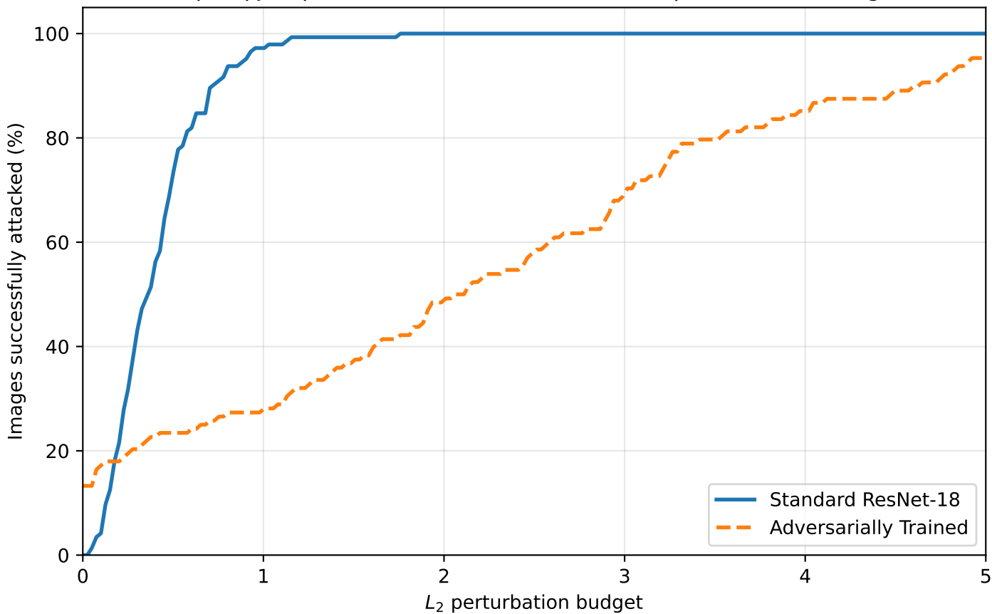
HopSkipJump: cumulative attack success vs perturbation budget
