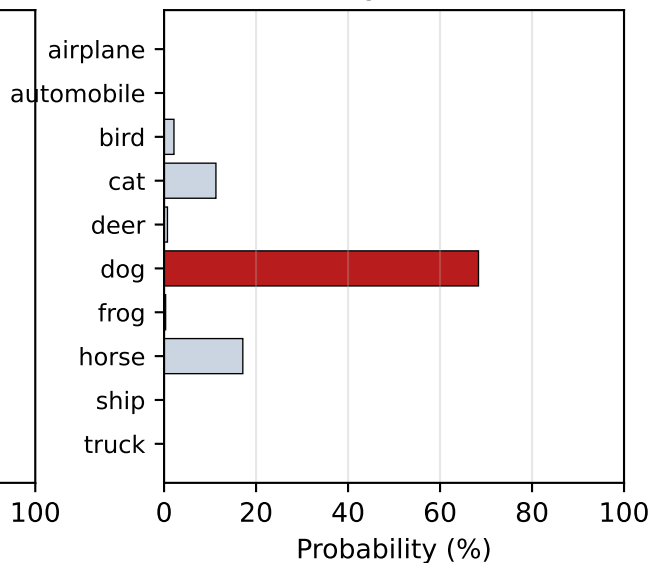
Robust Model
