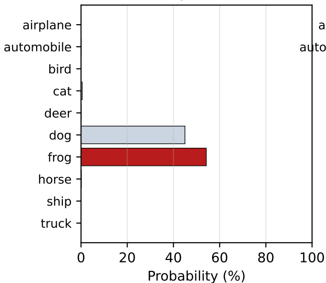
Standard Model
