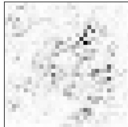
L_\infty norm: 0.0288
