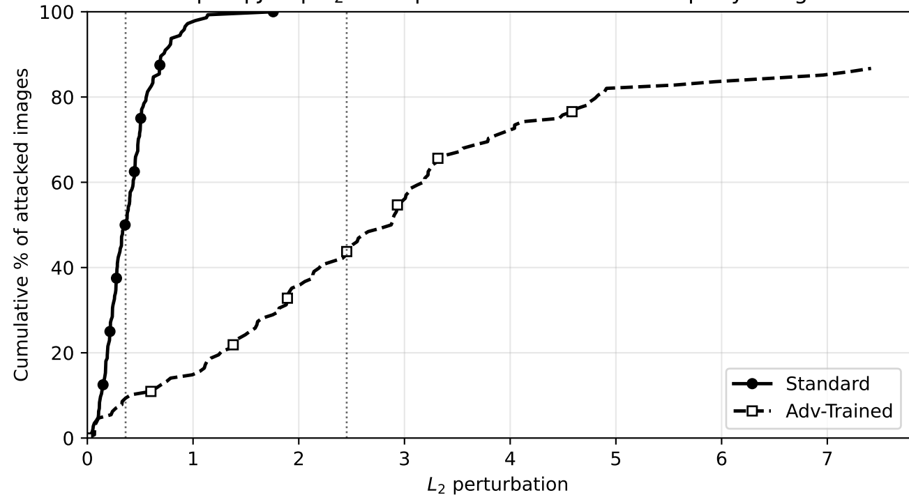
HopSkipJump L_2 : final perturbation within the query budget
