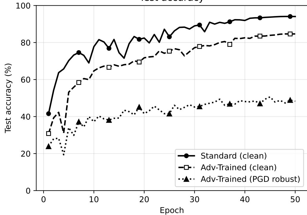
Test accuracy
