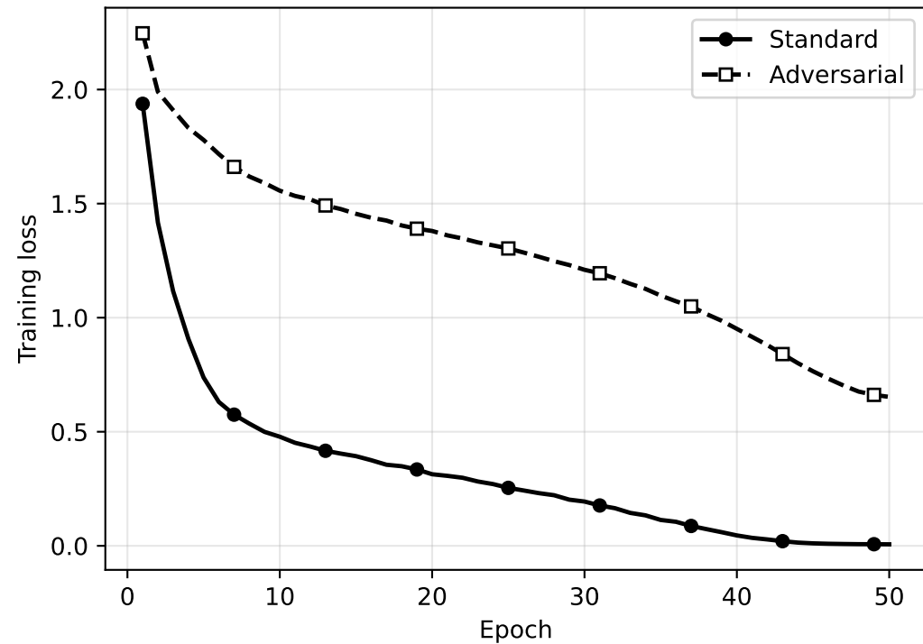
Training loss
