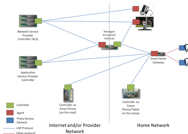
Figure 2 – USP Architecture Overview
