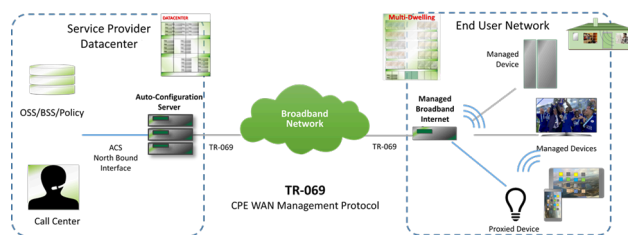
Figure 1 – CWMP Positioning in the End-to-End Architecture
