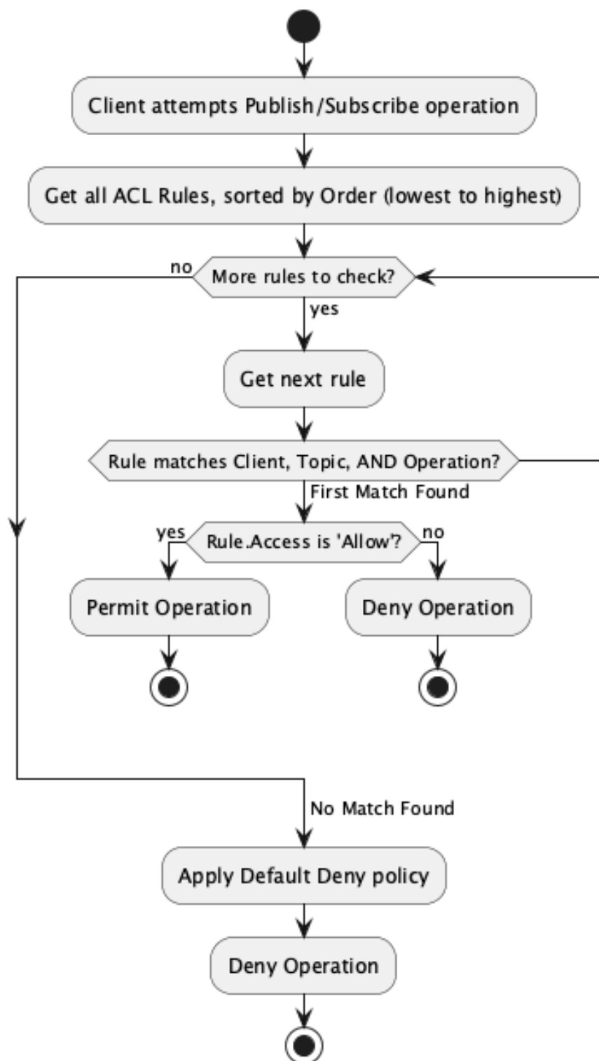
Figure 99 – MQTT ACL Evaluation Logic
