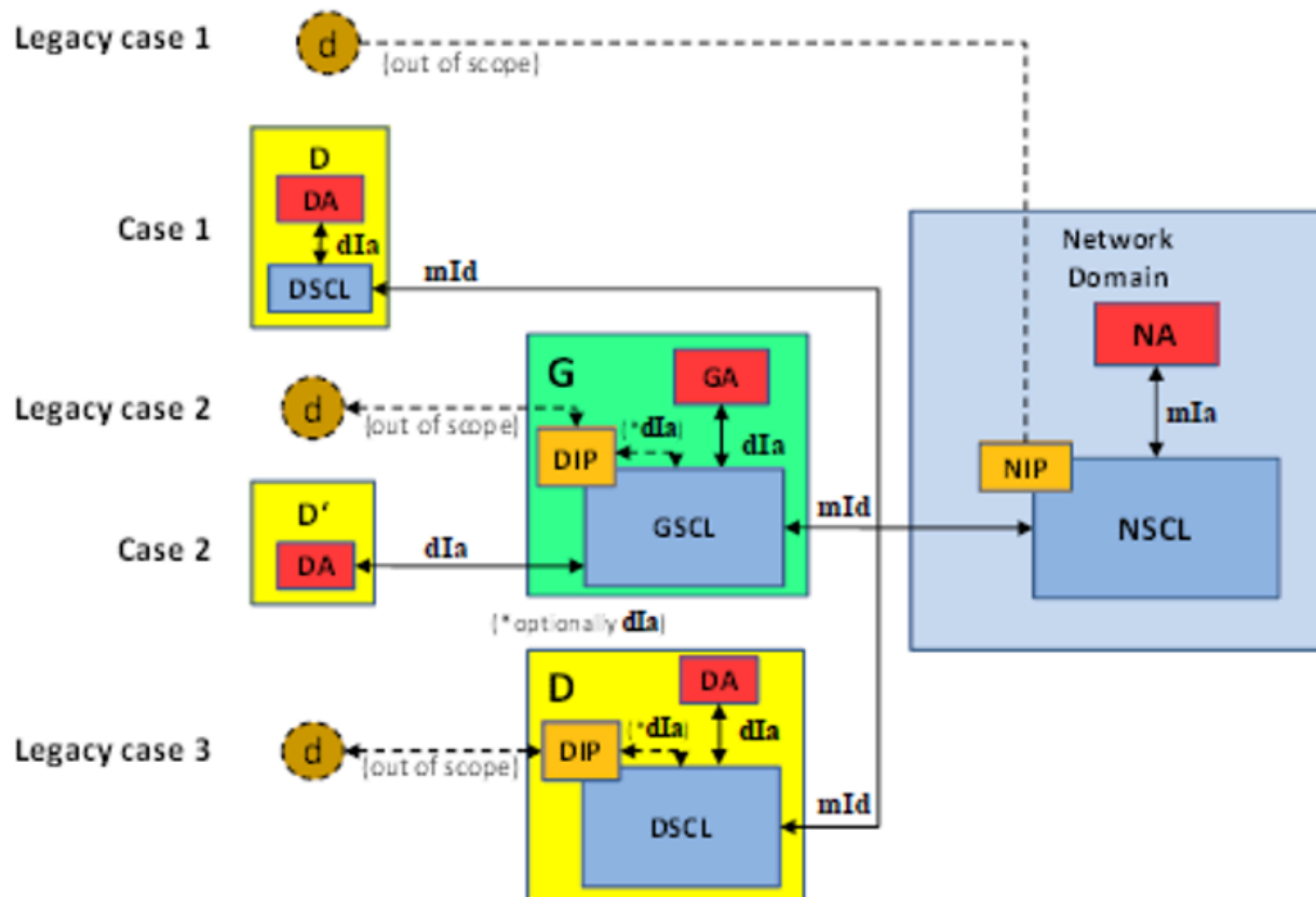
Figure 49 – ETSI M2M Devices and Gateways
