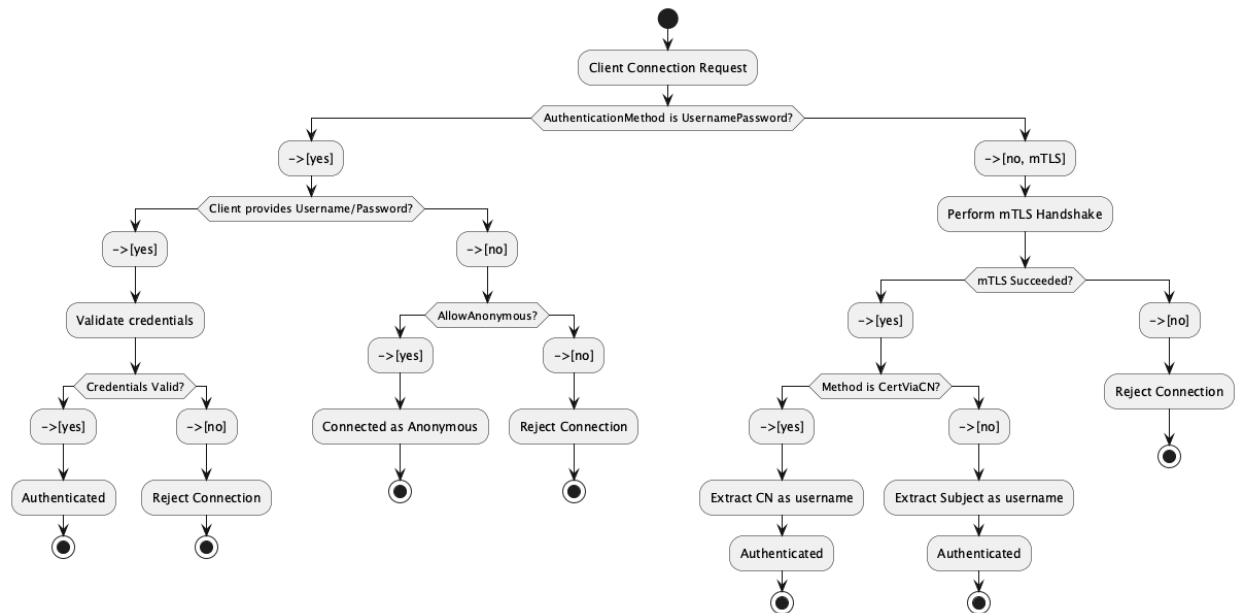
Figure 98 – MQTT Broker Authentication Flow
