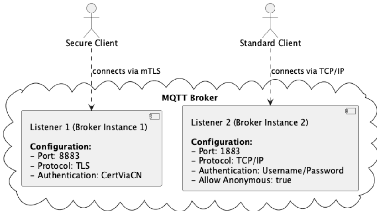
Figure 100 – MQTT Broker Listeners
