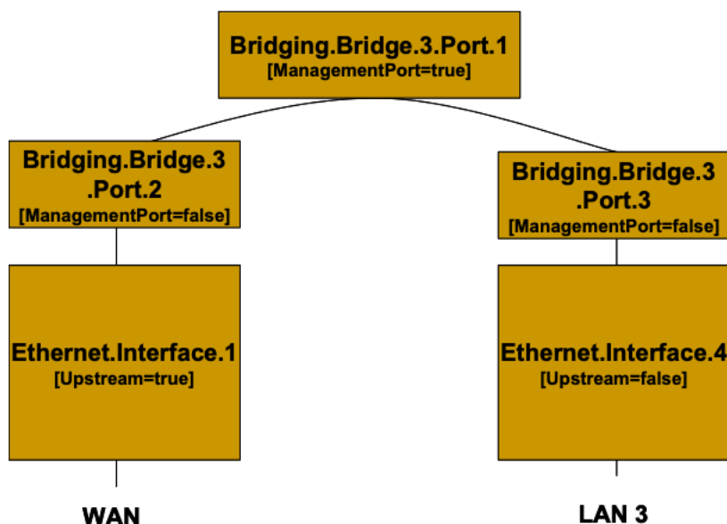
Figure 28 – Bridge 3 model
