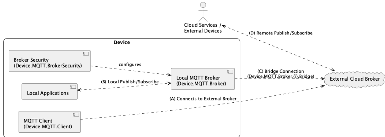
Figure 95 – MQTT Introduction Overview
