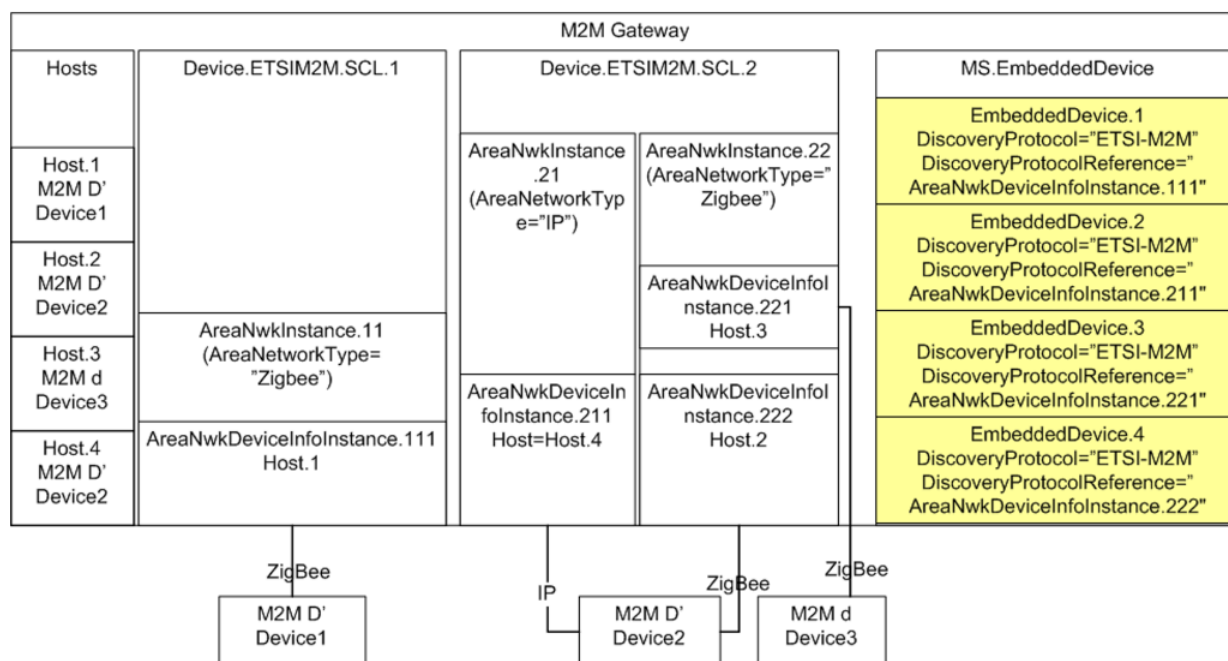
Figure 51 – M2M Device Discovery for Proxy Management
