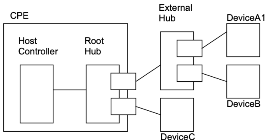
Figure 70 – Example USB Host Connections
