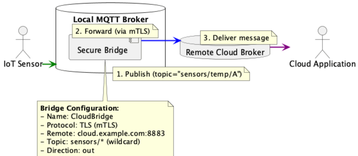
Figure 101 – MQTT Broker Bridge
