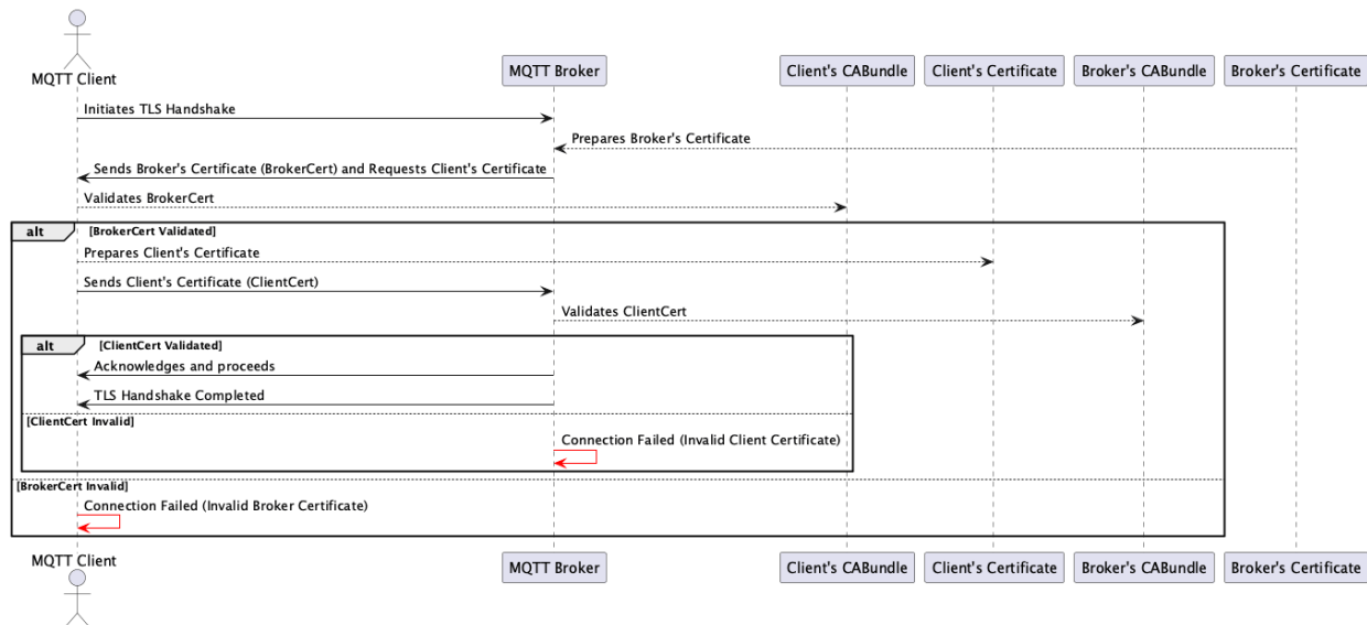
Figure 97 – MQTT Client Mutual Authentication TLS
