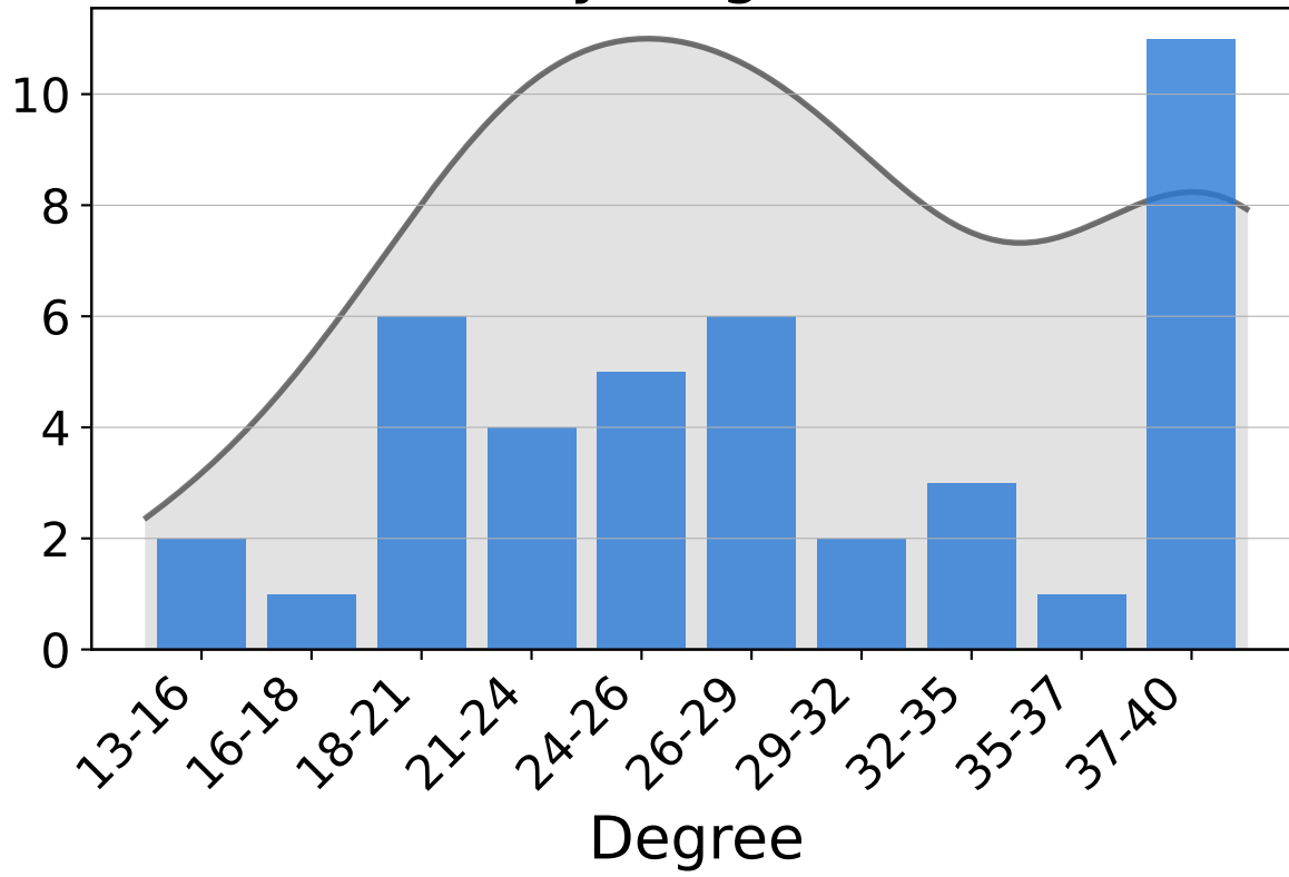
By Degree
