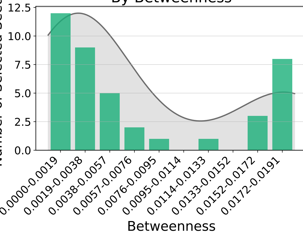
By Betweenness
