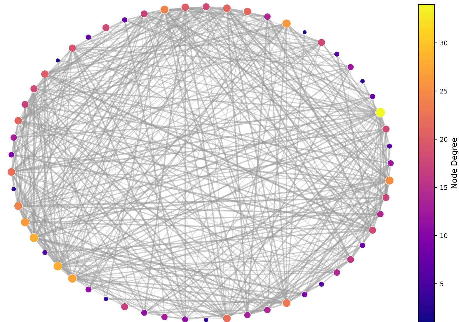
Contact Network bin 11 (57 nodes, 431 edges)
