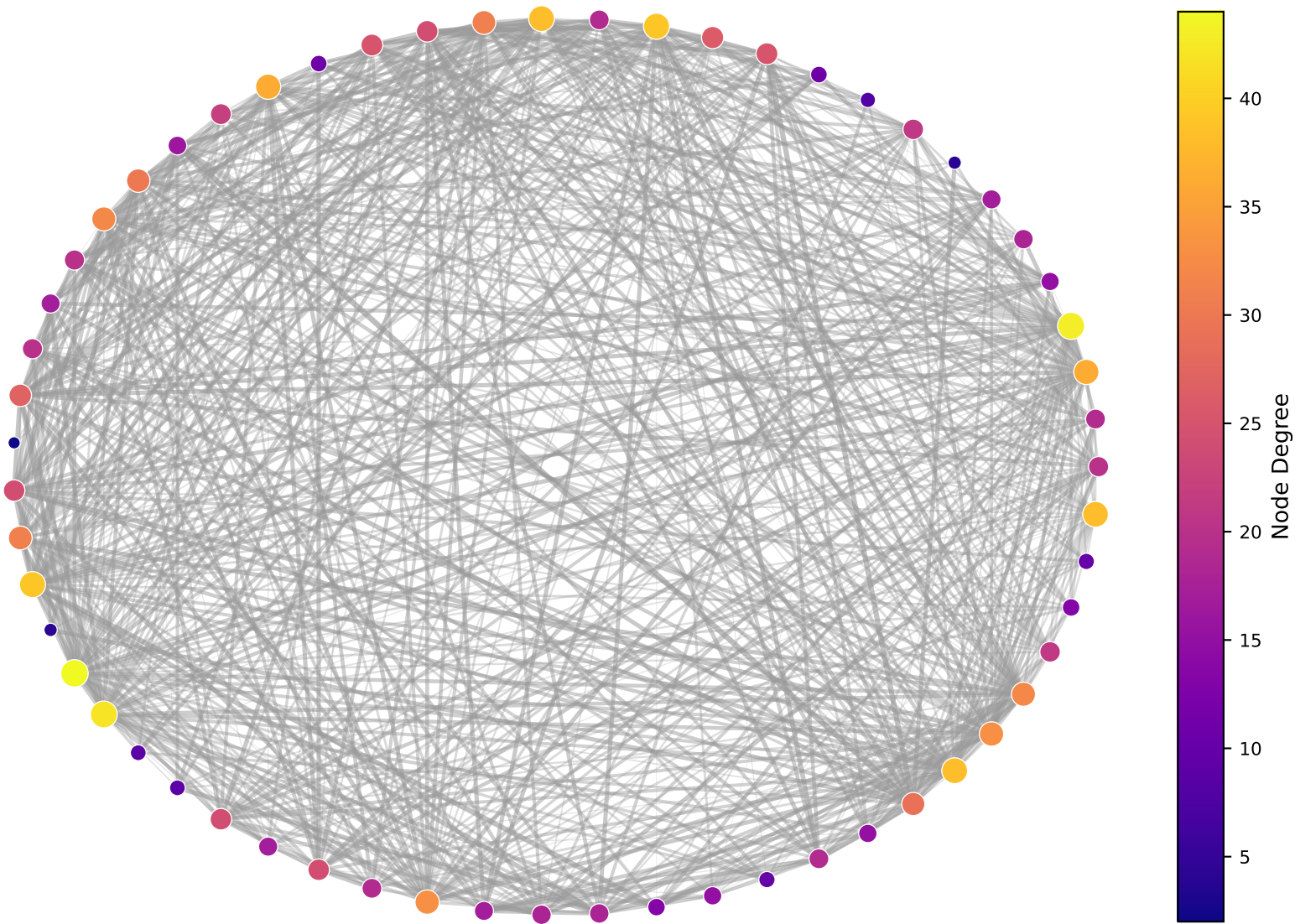
Contact Network bin 14 (59 nodes, 665 edges)
