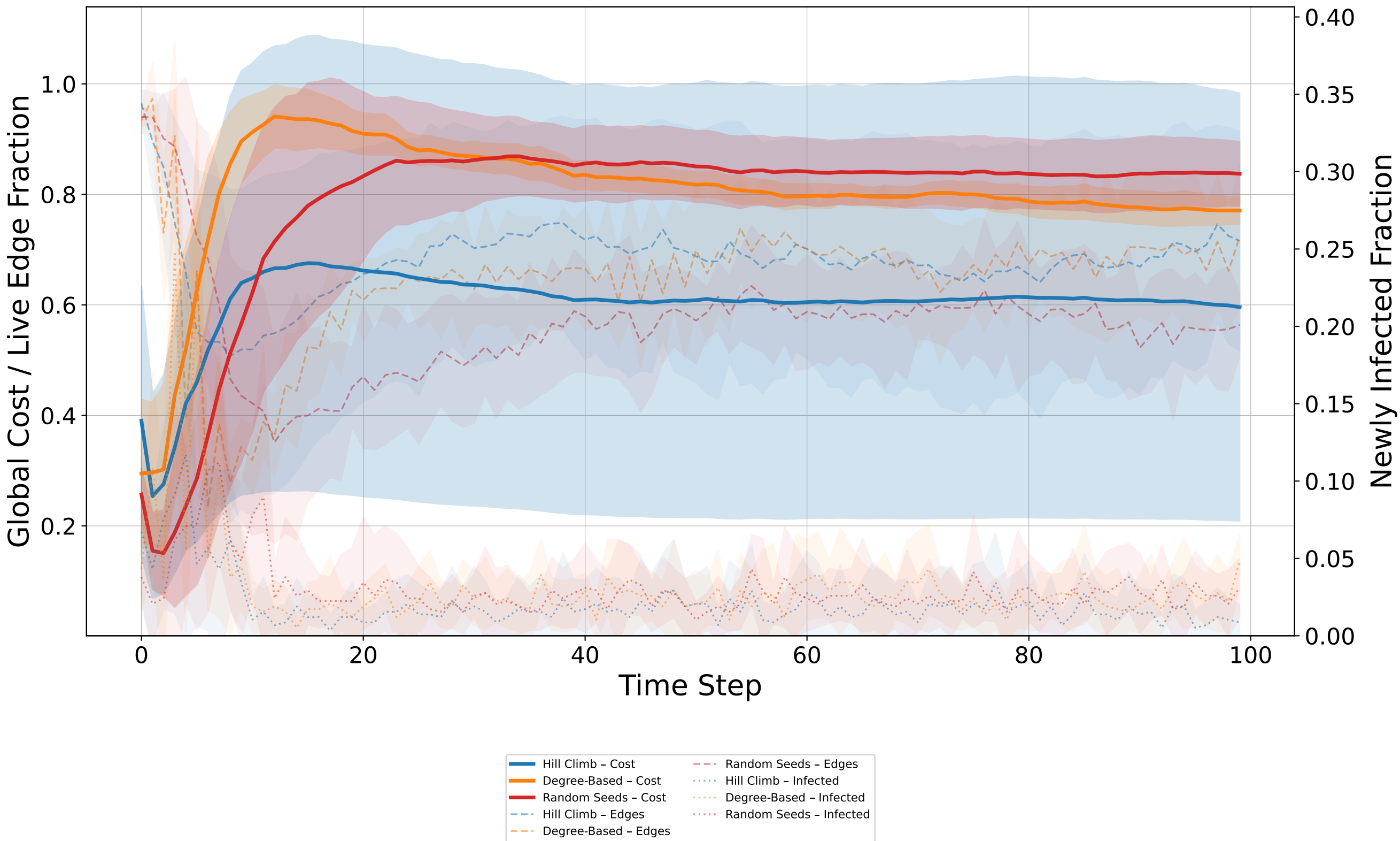
Method Comparison — bin 16
