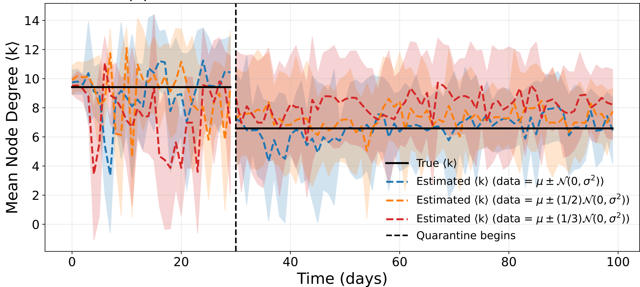
\langle k \rangle Estimation Under Gaussian Measurement Noise
