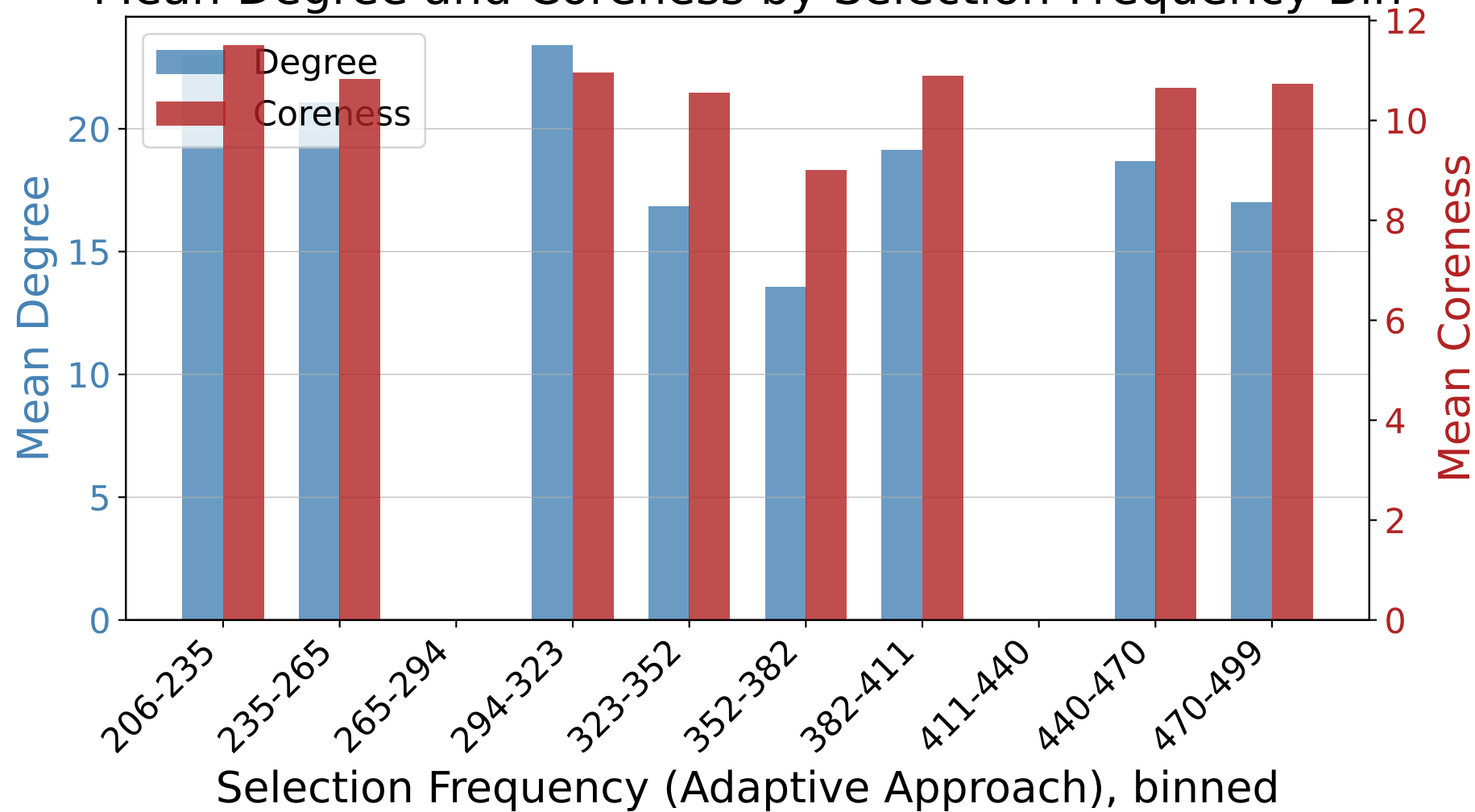
Mean Degree and Coreness by Selection-Frequency Bin
