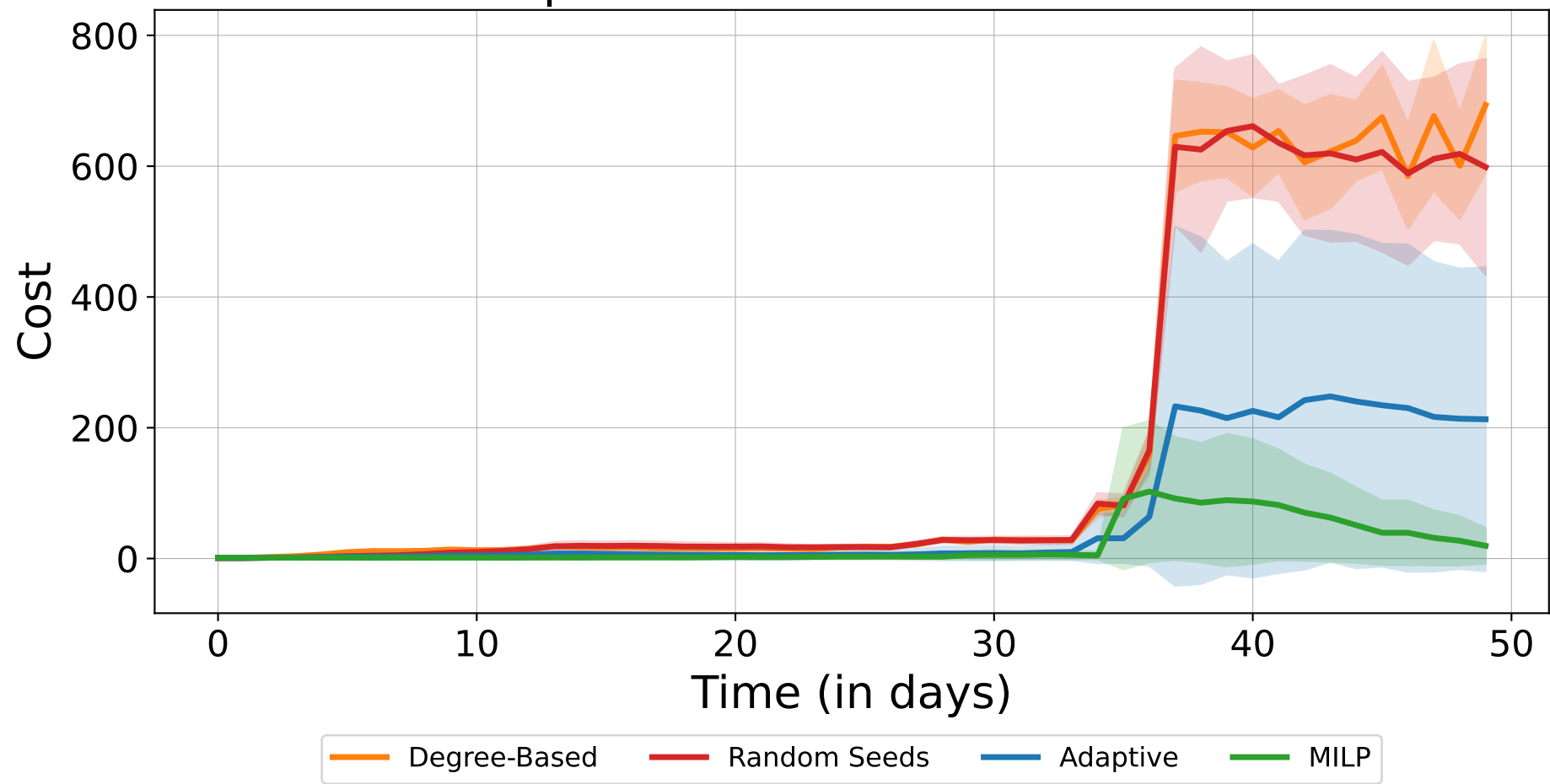
Cost Comparison of Seed Selection Methods
