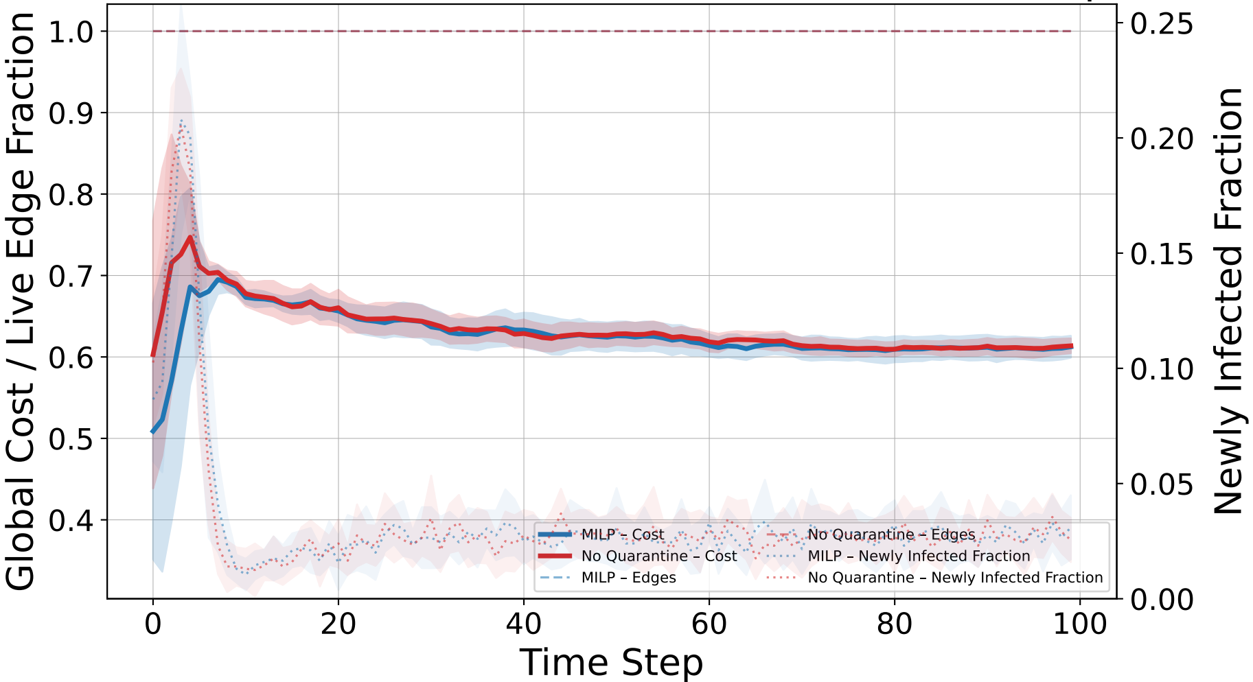
MILP Modified Network vs No Quarantine - Cost & Components
