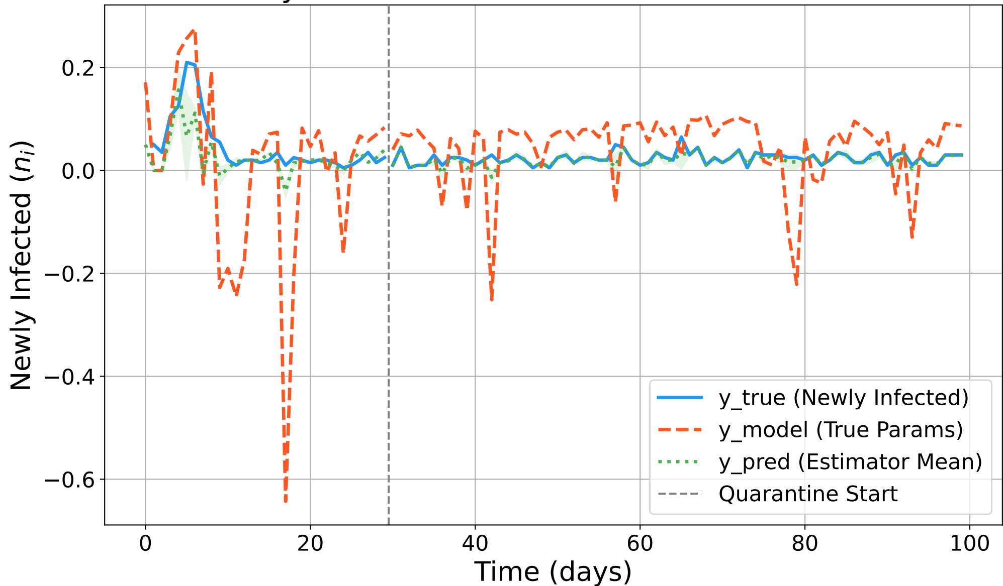
Identifiability Test: Estimator vs Model Eval with True Params
