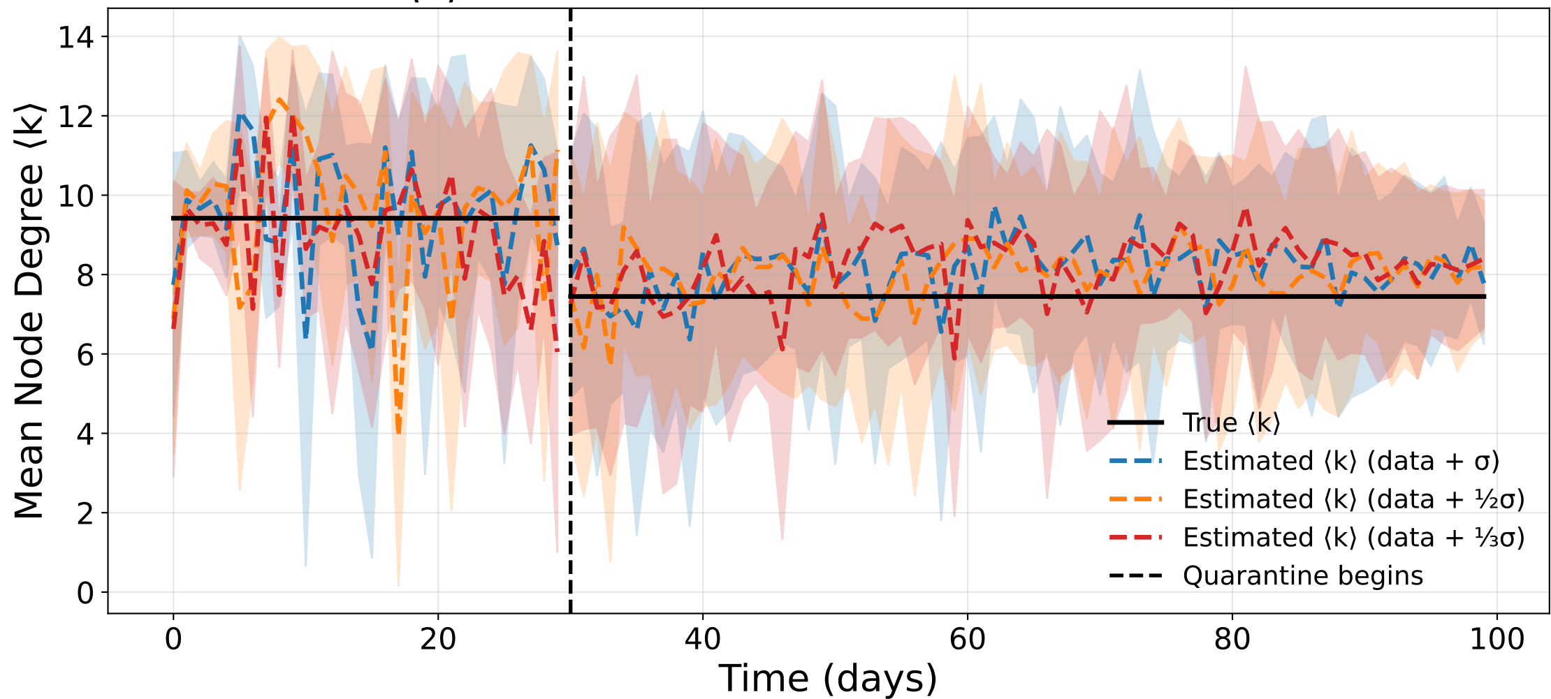
\langle k \rangle Estimation Under Measurement Noise
