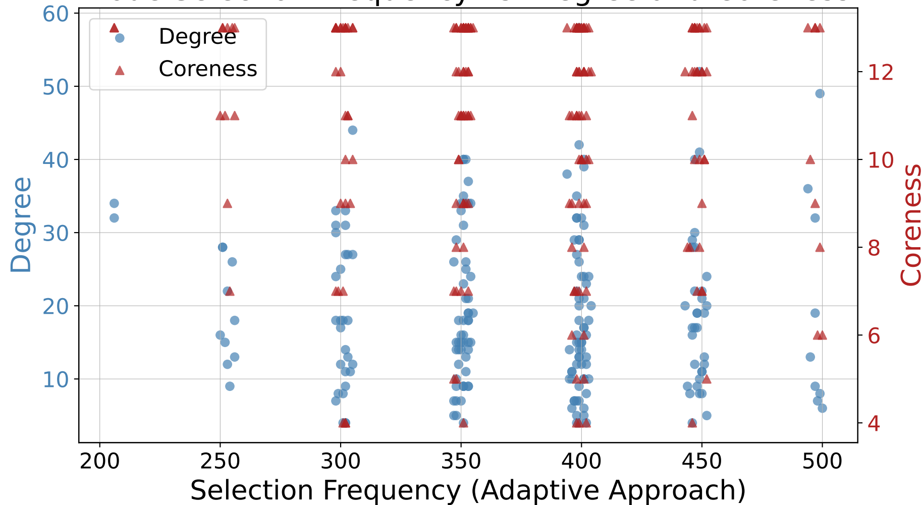
Node Selection Frequency vs. Degree and Coreness
