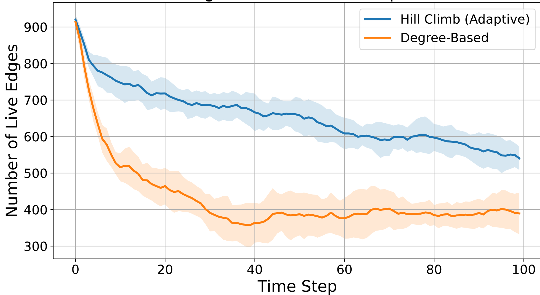
Live Edges Over Time - Comparison
