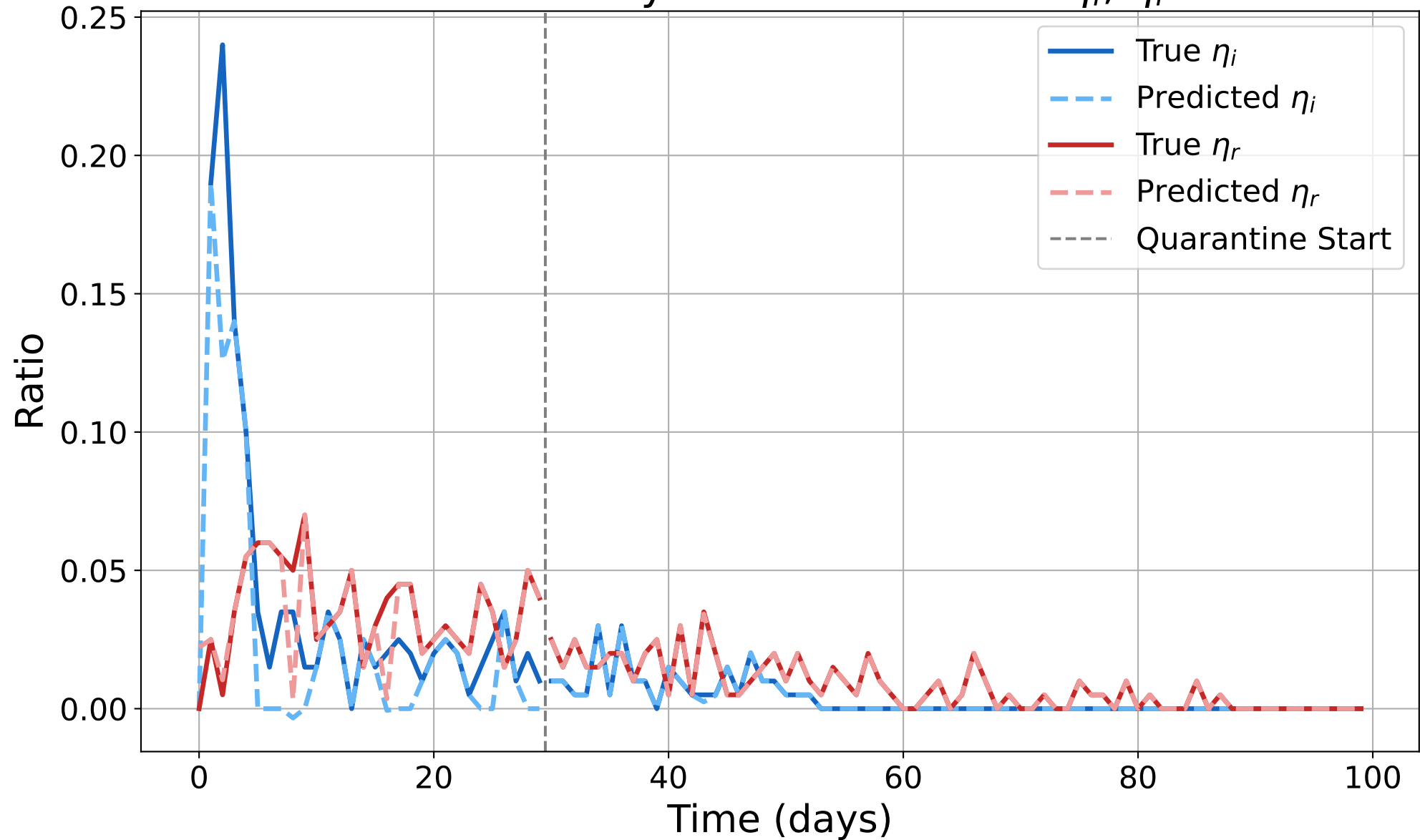
Identifiability: True vs Predicted \eta_i , \eta_r
