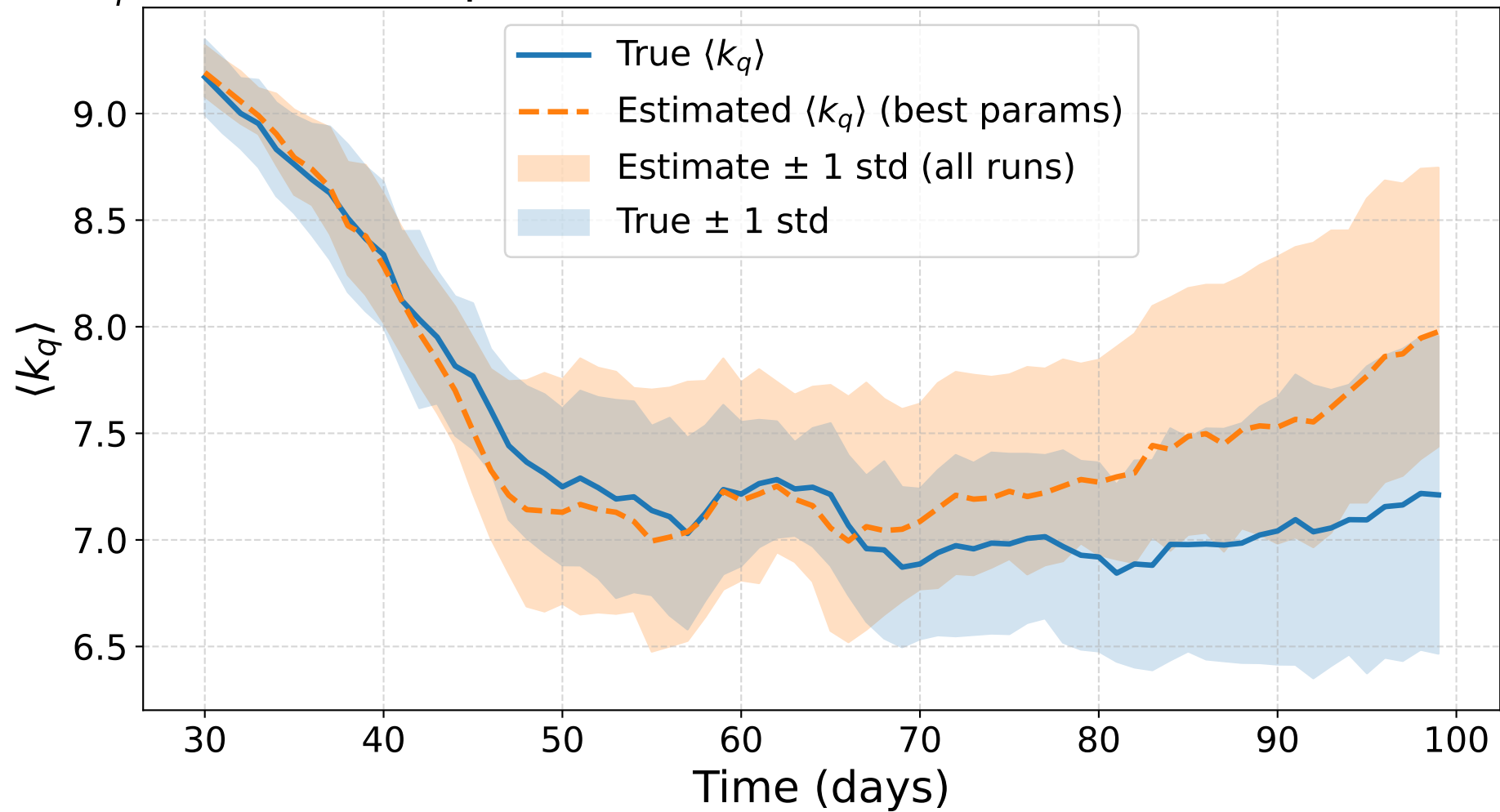
\langle k_q \rangle Parameter Optimization vs Ground Truth (adherence = 0.6)
