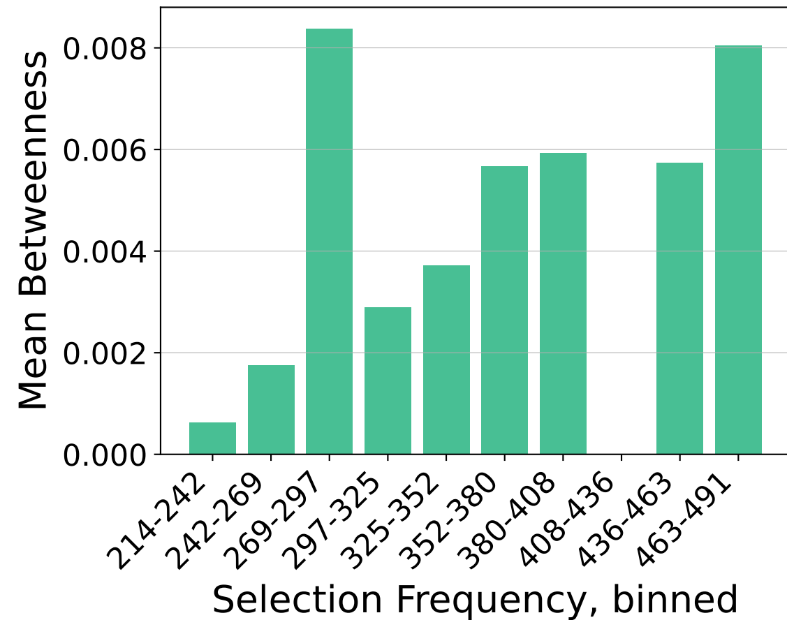
Betweenness
