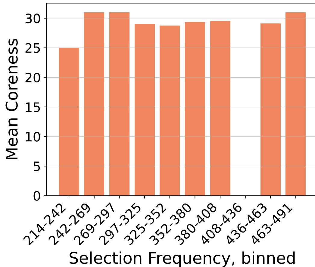
Coreness
