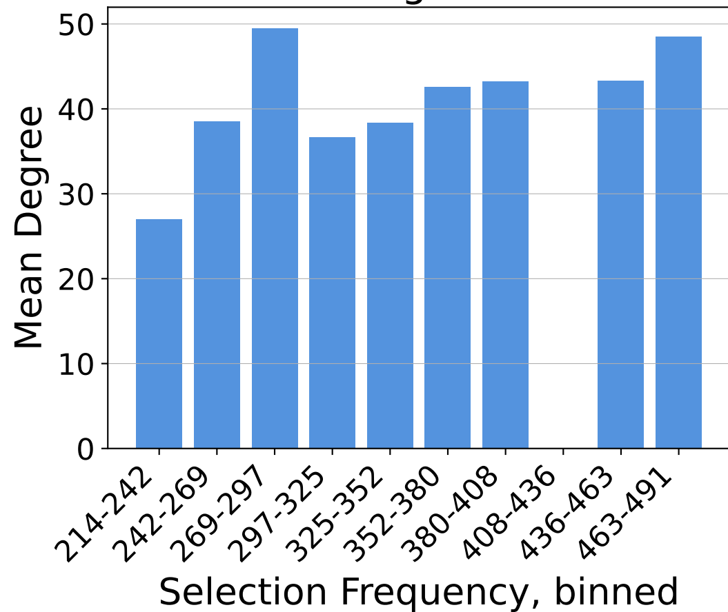
Degree
