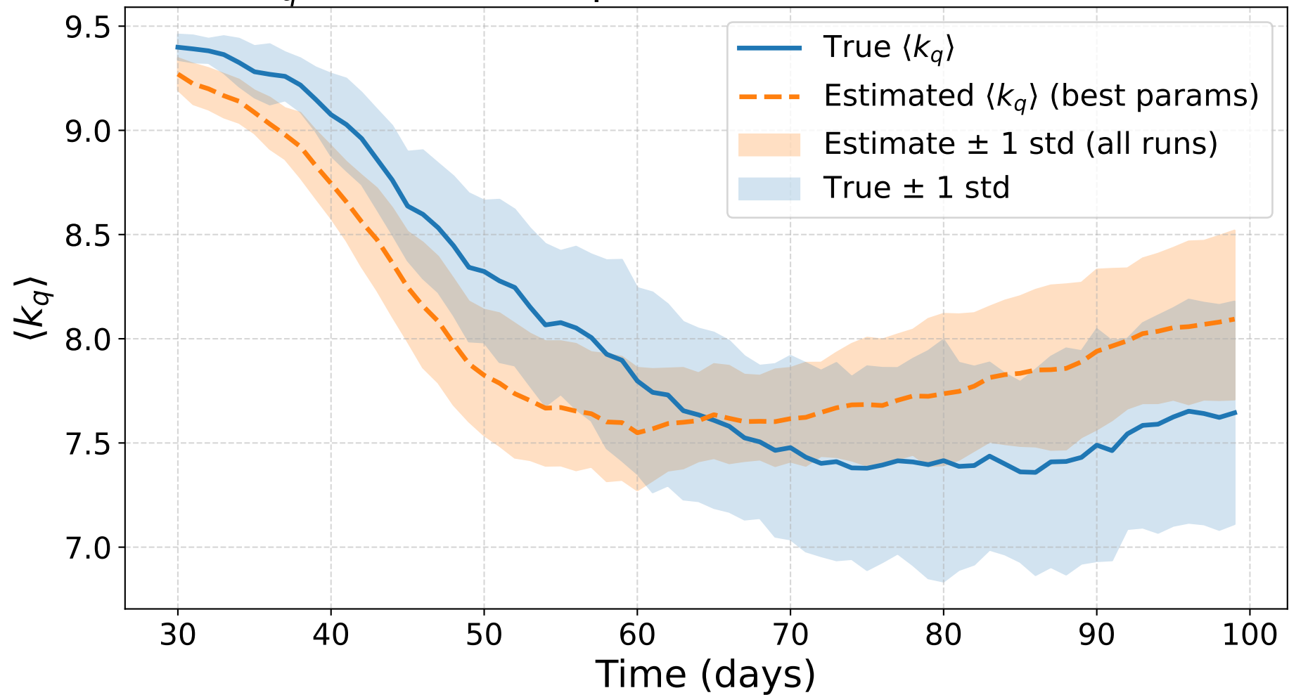
\langle k_q \rangle Parameter Optimization vs Ground Truth
