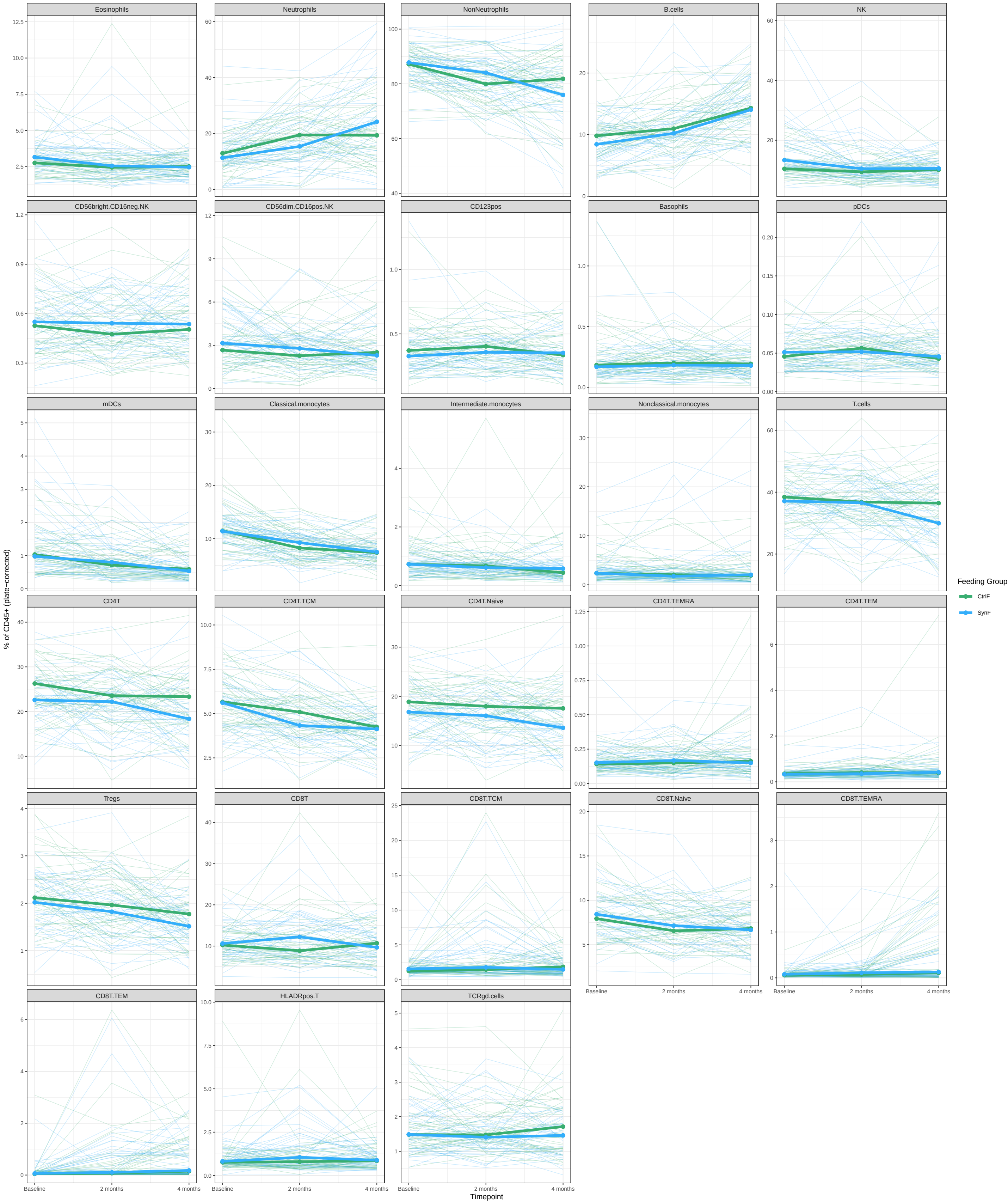
Manually-gated CyTOF populations over time: individual trajectories + group medians
