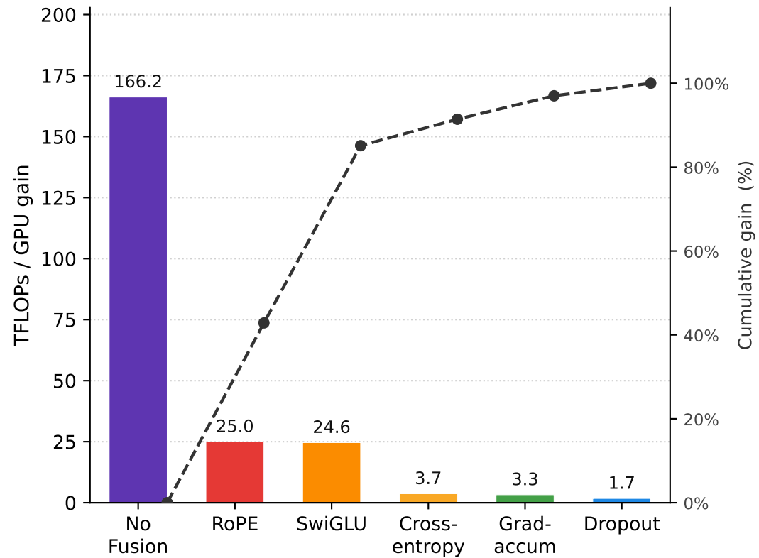
TFLOPs / GPU
