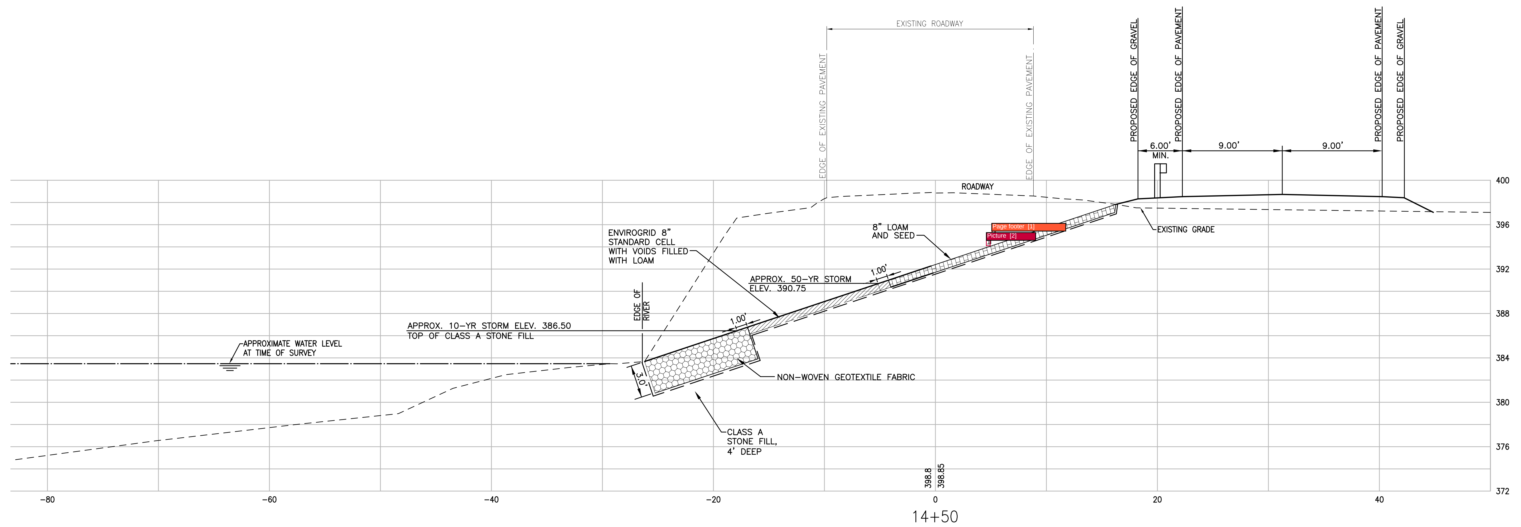
RIVER BED STABILIZATION SECTION - OPTION NO. 7
