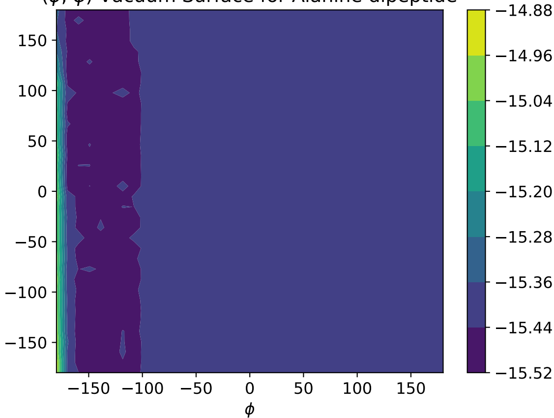
(\phi, \psi) Vacuum Surface for Alanine dipeptide
