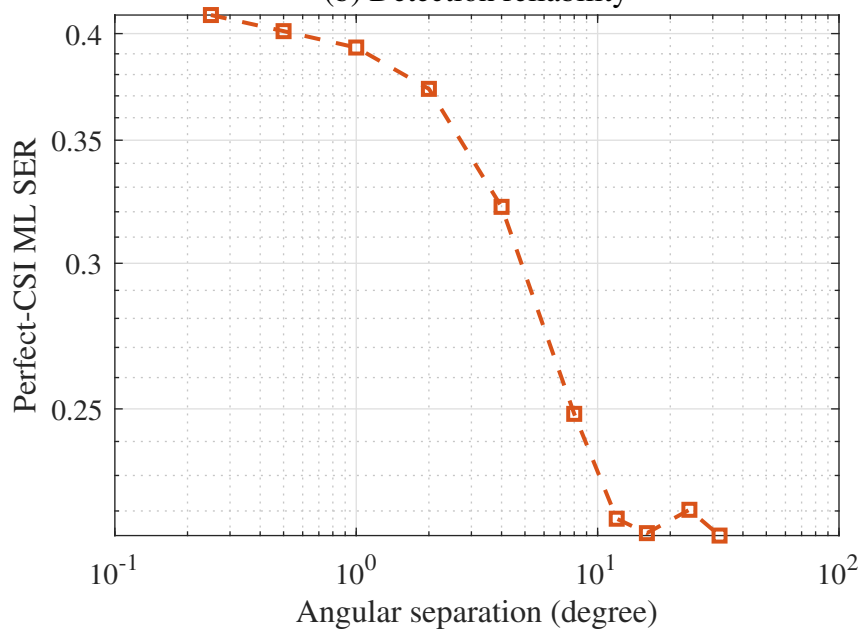
(b) Detection reliability
