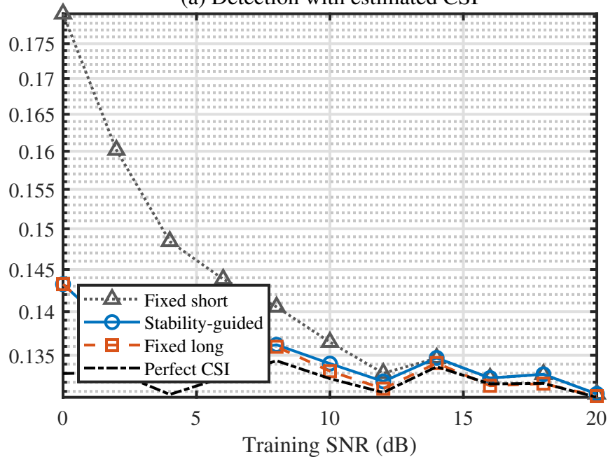
(a) Detection with estimated CSI
