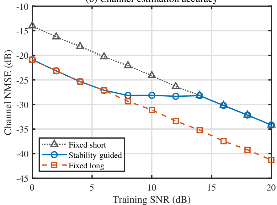
(b) Channel-estimation accuracy
