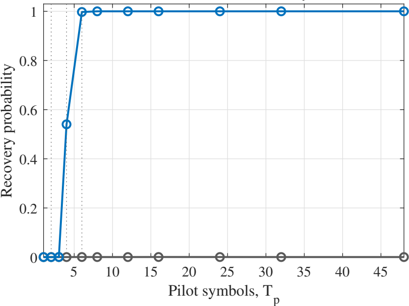
(a) Noiseless identifiability
