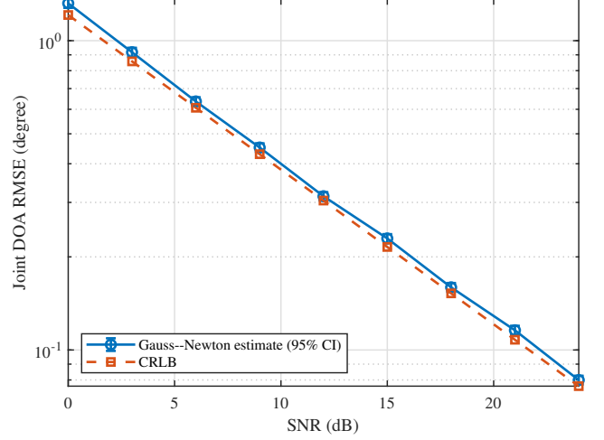
Fig. 2. Joint DOA RMSE and the corresponding CRLB versus SNR.
