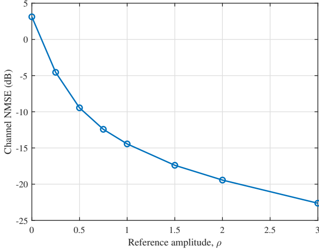
Fig. 4. Channel-estimation NMSE versus reference amplitude for fixed post-detection noise variance.
