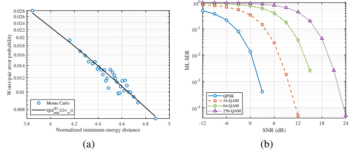
Fig. 7. Finite-alphabet reliability under perfect CSI: (a) worst-pair error probability versus normalized energy-domain minimum distance over equal-power fixed spatial phase maps and (b) exact-ML SER versus SNR for different unit-energy modulation alphabets under the fixed spatial four-phase reference map.
