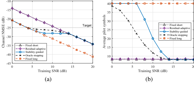
Fig. 5. Stability-guided adaptive training with the practical Algorithm 1 initialization: (a) channel NMSE and (b) average selected pilot symbols versus training SNR. The fixed-short and fixed-long schemes use T_p = 8 and 40, respectively; oracle stopping uses the true channel error only as an unattainable benchmark. Each point averages 300 paired trials.
