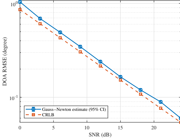
Fig. 3. Per-angle DOA RMSE and the corresponding root CRLB versus SNR under the fixed spatial four-phase reference code. Error bars show 95% confidence intervals.
