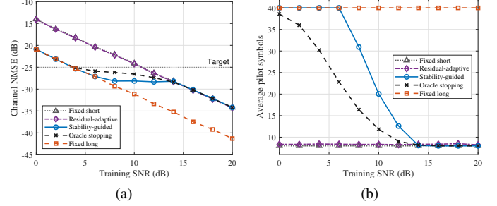
Fig. 5. Stability-guided adaptive training versus SNR: (a) channel NMSE and (b) average selected pilot length.
