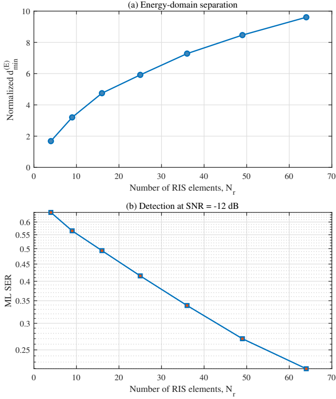
Fig. 13: Effect of the number of RIS element-level observations on (a) the normalized energy-domain minimum distance and (b) ML detection.
