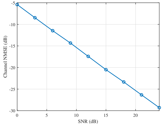
Fig. 2: Channel-estimation NMSE versus intensity-domain SNR.
