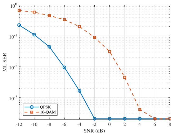
Fig. 10: ML SER for QPSK and 16-QAM under perfect CSI.
