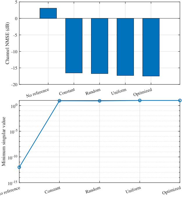
Fig. 6: Channel NMSE and minimum Jacobian singular value for different reference designs.
