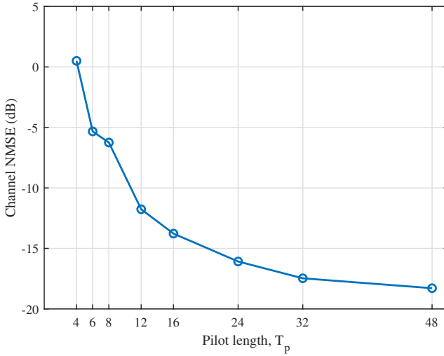
Fig. 4: Channel-estimation NMSE versus pilot length at an SNR of 12 dB.
