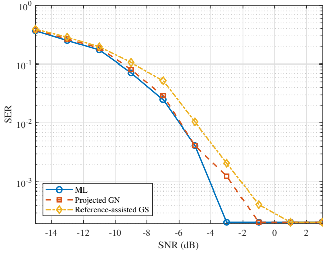
Fig. 7: SER of different symbol detectors under perfect CSI.
