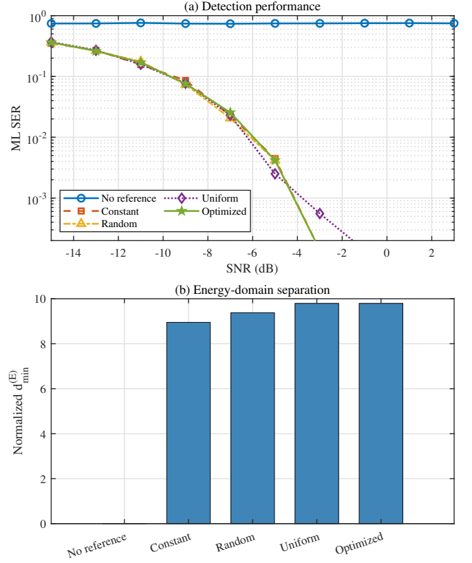
Fig. 8: Effect of the data-phase reference: (a) ML SER and (b) normalized energy-domain minimum distance.
