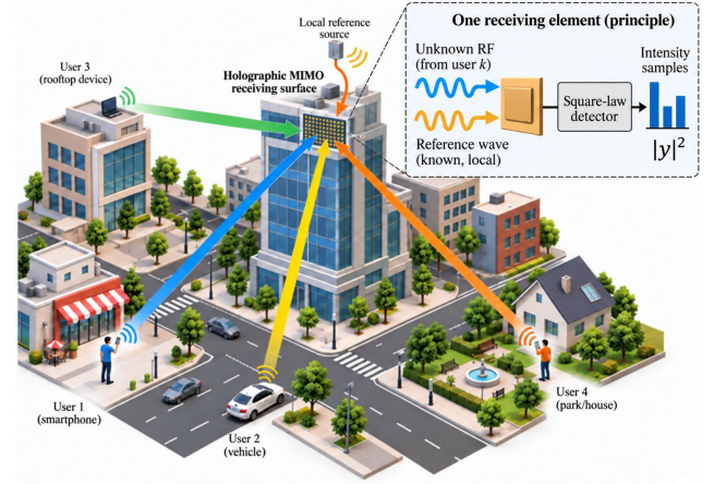
Fig. 1. Illustration of the proposed multi-user reference-assisted RF holographic reception architecture with intensity-only measurements.
