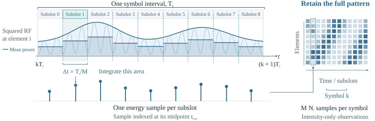
Fig. 2. Reference-assisted holographic reception model. Finite-alphabet symbols are pulse-shaped and upconverted to RF signals. After far-field propagation, the incident fields from different users form direction-dependent phase patterns across the holographic aperture. A known reference wave is added at the RF front end before square-law detection, converting relative phase information into intensity variations. When waveform variation within a symbol must be resolved, the symbol interval is divided into M subslots; otherwise, M = 1 . The receiver preserves the resulting spatial intensity pattern for channel estimation and symbol detection.
