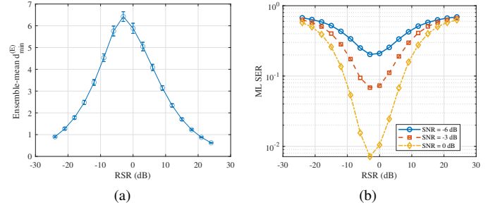
Fig. 11. Effect of the reference-to-signal energy ratio under a fixed total incident-energy budget: (a) ensemble-mean minimum energy distance over phase-balanced spatial maps and (b) perfect-CSI ML SER at three balanced-case SNRs. Error bars show one standard deviation across phase maps.
