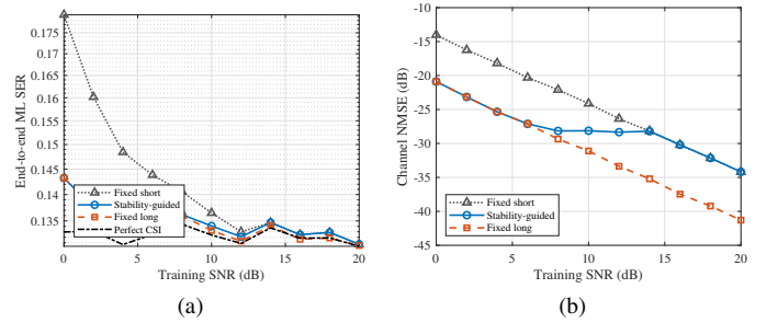
Fig. 8. End-to-end comparison versus training SNR: (a) SER of the fixed-short, stability-guided, and fixed-long training policies with perfect-CSI ML as a benchmark and (b) their channel NMSE. The data SNR is 0 dB.
