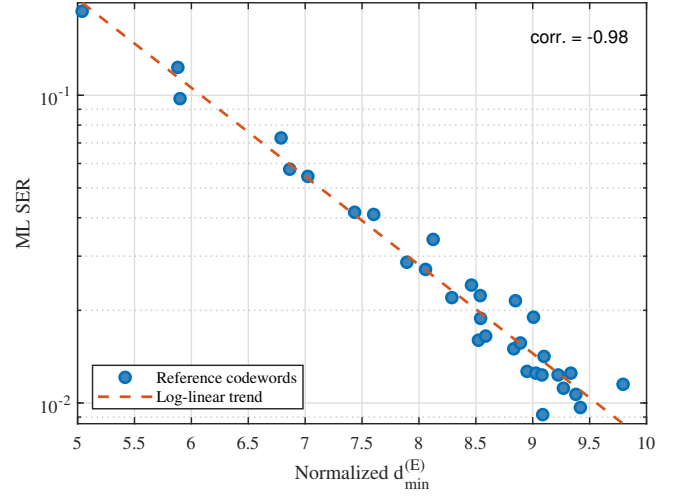
Fig. 8. ML SER versus normalized energy-domain minimum distance over an equal-power reference codebook.
