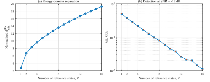
Fig. 13. Effect of the number of phase-shifted reference states on (a) the normalized energy-domain minimum distance and (b) ML detection.
