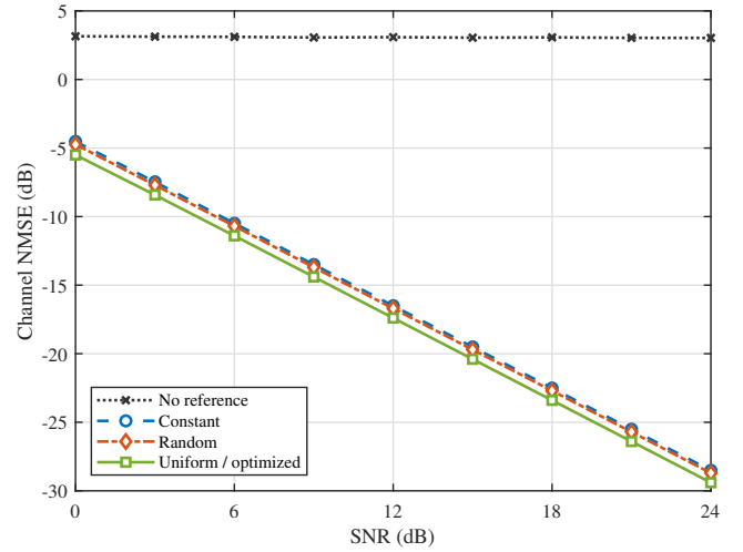
Fig. 5. Channel-estimation NMSE versus SNR for different training-reference designs.
