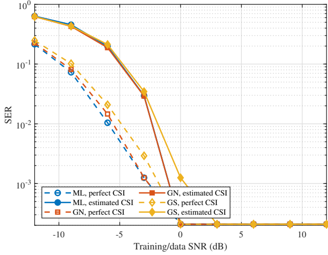
Fig. 10. SER under perfect and estimated CSI for different symbol detectors.
