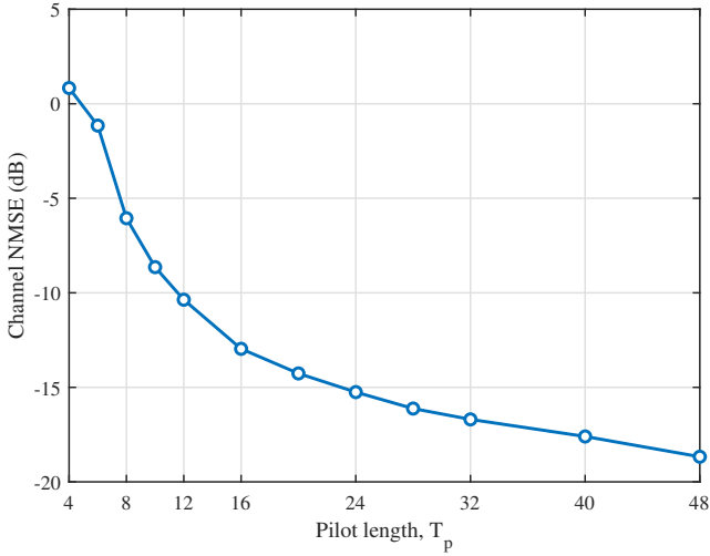
Fig. 3. Channel-estimation NMSE versus pilot length at an SNR of 12 dB.
