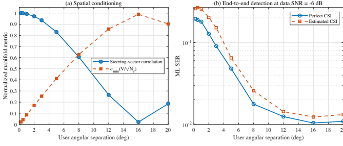
Fig. 14. Effect of user angular separation on (a) array-manifold conditioning and (b) end-to-end ML detection.
