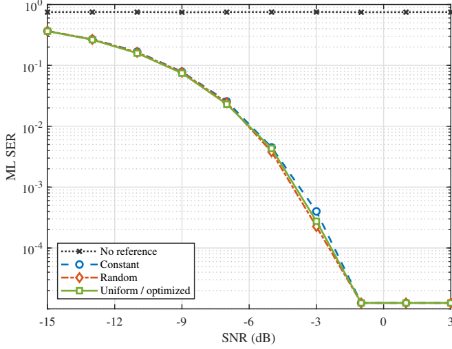
Fig. 7. ML SER versus SNR for different data-phase reference designs under perfect CSI. Zero-error points are displayed at the half-event level.
