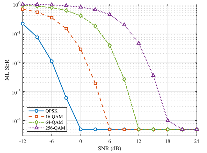
Fig. 9. ML SER for QPSK, 16-QAM, 64-QAM, and 256-QAM under perfect CSI. Zero-error points are displayed at the half-event level.
