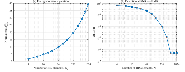
Fig. 12. Effect of the number of RIS element-level observations on (a) the normalized energy-domain minimum distance and (b) ML detection at -12 dB. Zero-error points are displayed at the half-event level.
