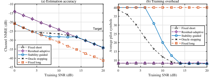
Fig. 5. Stability-guided adaptive training with the practical Algorithm 1 initialization: (a) channel NMSE and (b) average selected pilot symbols versus training SNR. The fixed-short and fixed-long schemes use T_p = 8 and 40, respectively; oracle stopping uses the true channel error only as an unattainable benchmark. Each point averages 300 paired trials.
