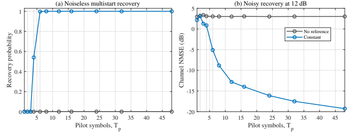
Fig. 4. Effect of pilot count for the two-user unstructured training problem: (a) empirical noiseless multistart recovery probability and (b) channel NMSE at 12 dB, with and without a fixed nonzero reference. The vertical lines mark T_p = L, 2L , and 3L .
