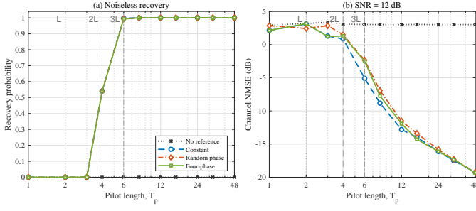
Fig. 4. Effect of pilot count and reference design for the two-user unstructured training problem: (a) empirical noiseless multistart recovery probability and (b) channel NMSE at 12 dB. The vertical lines mark T_p = L , 2L , and 3L .
