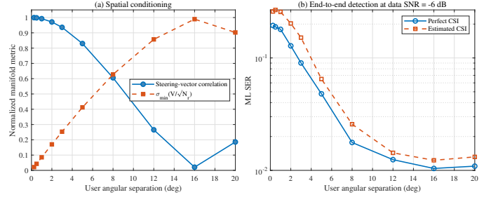
Fig. 10. Effect of user angular separation on (a) array-manifold conditioning and (b) end-to-end ML detection.
