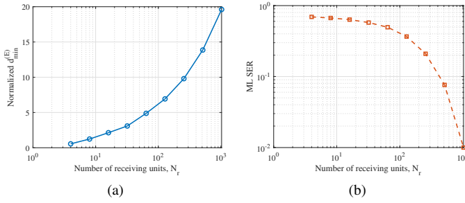
Fig. 9. Combined effect of receiving-surface size and observation count on (a) the normalized energy-domain minimum distance and (b) perfect-CSI ML detection at -12 dB.
