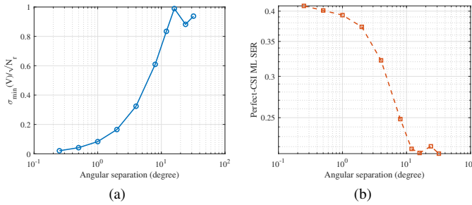
Fig. 10. Effect of user angular separation on (a) array-manifold conditioning and (b) perfect-CSI ML detection at -6 dB.
