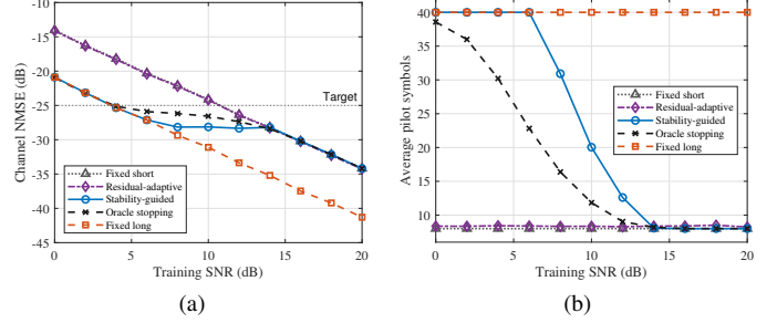
Fig. 5. Stability-guided adaptive training with the practical Algorithm 1 initialization: (a) channel NMSE and (b) average selected pilot symbols versus training SNR. The fixed-short and fixed-long schemes use T_p = 8 and 40, respectively; oracle stopping uses the true channel error only as an unattainable benchmark. Each point averages 300 paired trials.
