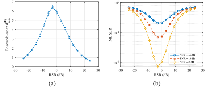
Fig. 11. Effect of the reference-to-signal energy ratio under a fixed total incident-energy budget: (a) ensemble-mean minimum energy distance over phase-balanced spatial maps and (b) perfect-CSI ML SER at three balanced-case SNRs. Error bars show one standard deviation across phase maps.
