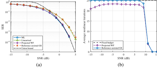
Fig. 6. Perfect-CSI detection: (a) SER of ML, linearized, projected-WF, and reference-assisted GS detectors together with the analytical distance-spectrum union bound, and (b) their average nonlinear iterations under the exact d_{\min}^{(E)} stopping certificate. Empirical SER points with no observed errors are omitted.
