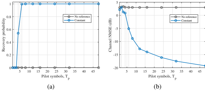
Fig. 4. Effect of pilot count for the two-user unstructured training problem: (a) empirical noiseless multistart recovery probability and (b) channel NMSE at 12 dB, with and without a fixed nonzero reference. The vertical lines mark T_p = L , 2L , and 3L .
