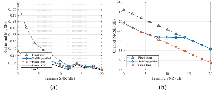
Fig. 8. End-to-end comparison versus training SNR: (a) SER of the fixed-short, stability-guided, and fixed-long training policies with perfect-CSI ML as a benchmark and (b) their channel NMSE. The data SNR is 0 dB.
