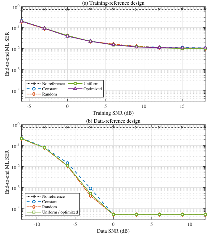
Fig. 12. End-to-end ML SER versus (a) training SNR for different training-reference designs at a data SNR of -6 dB and (b) data SNR for different data-reference designs at a training SNR of 12 dB. Zero-error points are displayed at the half-event level.
