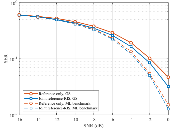
Fig. 16. SER of the proposed reference-assisted GS detector and the ML benchmark under equal-overhead reference-only and joint reference-RIS measurement diversity.
