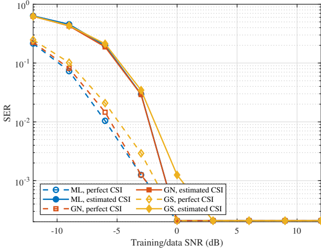
Fig. 11. SER under perfect and estimated CSI for different symbol detectors.
