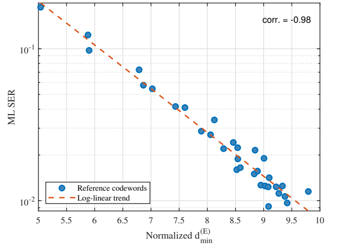
Fig. 9. ML SER versus normalized energy-domain minimum distance over an equal-power reference codebook.
