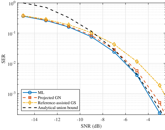
Fig. 7. SER of different symbol detectors under perfect CSI, averaged over 10^5 trials per SNR, and the analytical distance-spectrum union bound.
