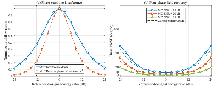
Fig. 17. Effect of the reference-to-signal energy ratio under a fixed total incident-energy budget: (a) normalized interference depth and relative phase information and (b) phase RMSE of four-phase field recovery. Solid curves with markers are Monte Carlo results, dashed curves are the corresponding CRLBs, and the horizontal dotted line denotes a 10^\circ RMSE criterion.
