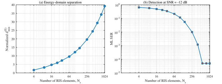
Fig. 13. Effect of the number of RIS element-level observations on (a) the normalized energy-domain minimum distance and (b) ML detection at -12 dB. Zero-error points are displayed at the half-event level.
