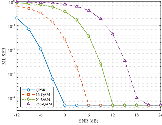
Fig. 10. ML SER for QPSK, 16-QAM, 64-QAM, and 256-QAM under perfect CSI. Zero-error points are displayed at the half-event level.
