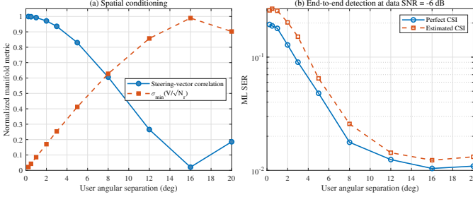
Fig. 15. Effect of user angular separation on (a) array-manifold conditioning and (b) end-to-end ML detection.
