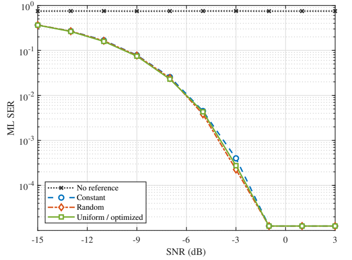
Fig. 8. ML SER versus SNR for different data-phase reference designs under perfect CSI. Zero-error points are displayed at the half-event level.
