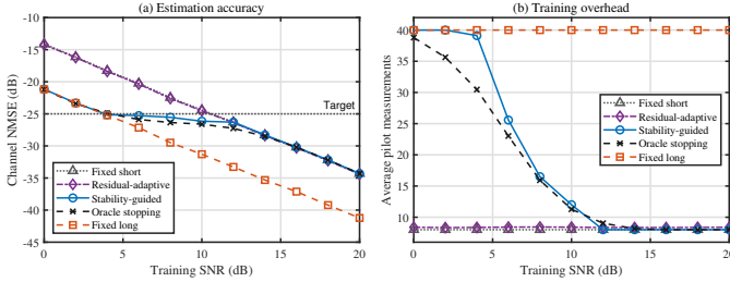
Fig. 5. Stability-guided adaptive training with the practical Algorithm 1 initialization: (a) channel NMSE and (b) average selected pilot measurements versus training SNR. The fixed-short and fixed-long schemes use T_p = 8 and 40, respectively; oracle stopping uses the true channel error only as an unattainable benchmark. Each point averages 1000 paired trials.
