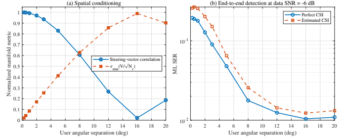
Fig. 10. Effect of user angular separation on (a) array-manifold conditioning and (b) end-to-end ML detection.
