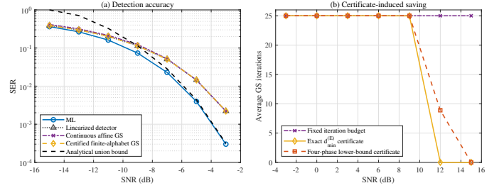
Fig. 6. Perfect-CSI detection: (a) SER of ML, linearized, and GS detectors together with the analytical distance-spectrum union bound, and (b) average GS back-projections with a fixed budget, the exact d_{\min}^{(E)} certificate, and the four-phase lower-bound certificate.
