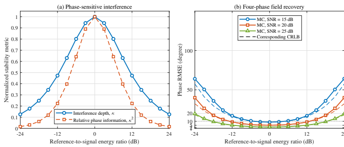
Fig. 11. Effect of the reference-to-signal energy ratio under a fixed total incident-energy budget: (a) normalized interference depth and relative phase information and (b) phase RMSE of four-phase field recovery. Solid curves with markers are Monte Carlo results, dashed curves are the corresponding CRLBs, and the horizontal dotted line denotes a 10^\circ RMSE criterion.
