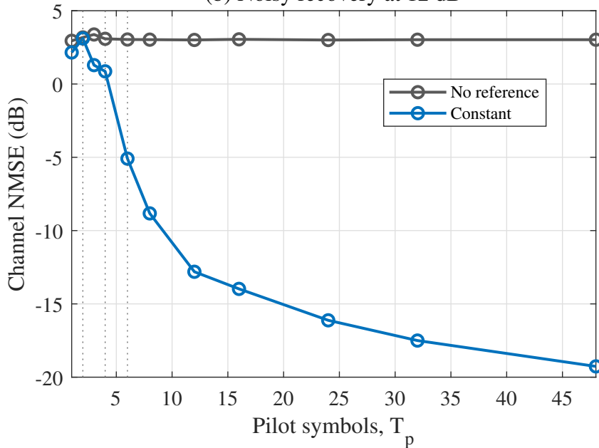
(b) Noisy recovery at 12 dB
