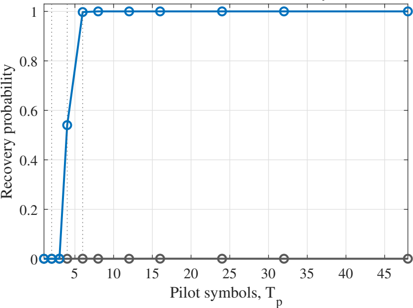
(a) Noiseless multistart recovery
