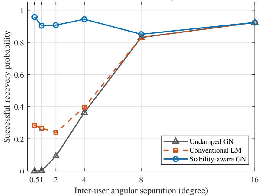
(b) Basin reliability
