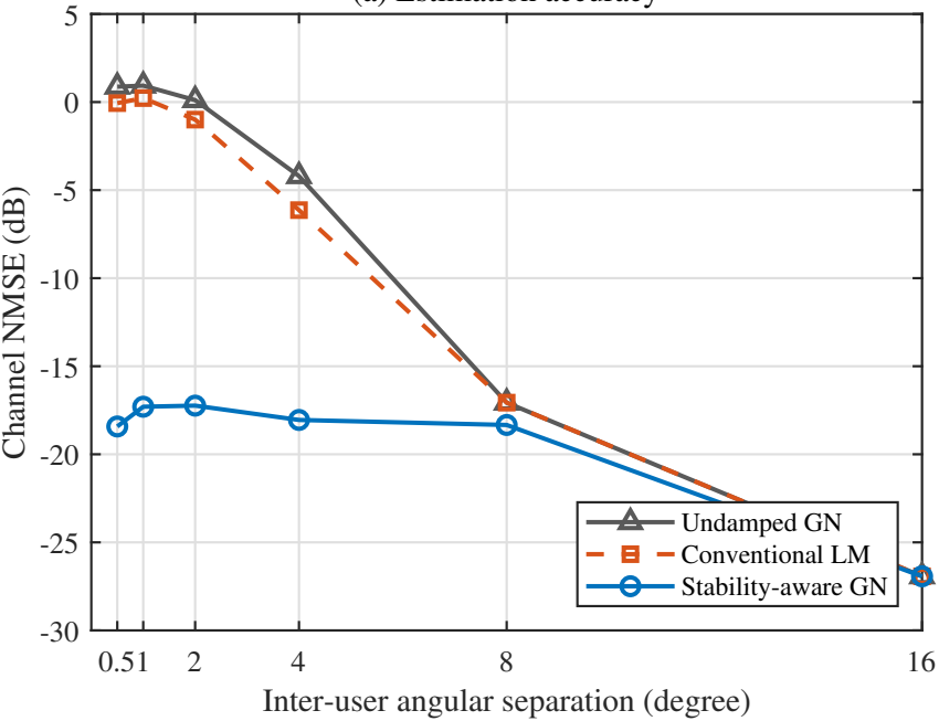
(a) Estimation accuracy
