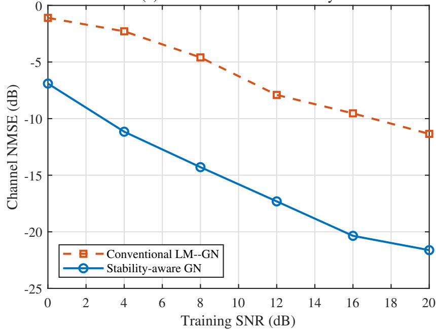
(b) Channel-estimation accuracy
