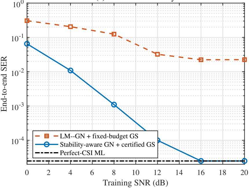
(a) Detection reliability
