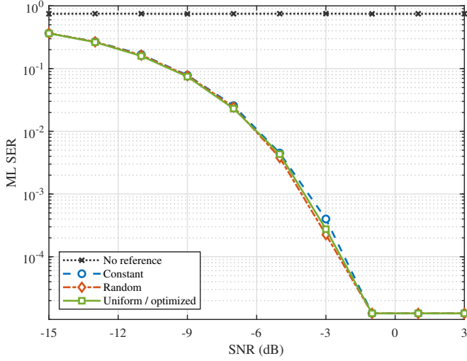
Fig. 8. ML SER versus SNR for different data-phase reference designs under perfect CSI. Zero-error points are displayed at the half-event level.
