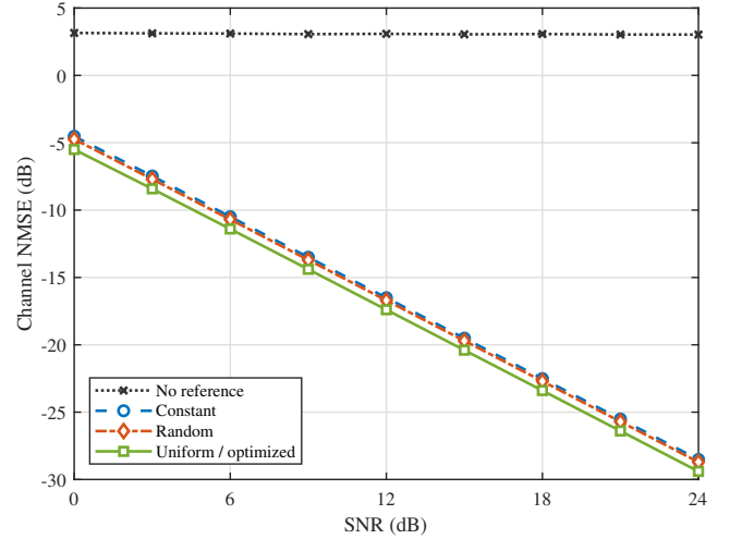
Fig. 6. Channel-estimation NMSE versus SNR for different training-reference designs.
