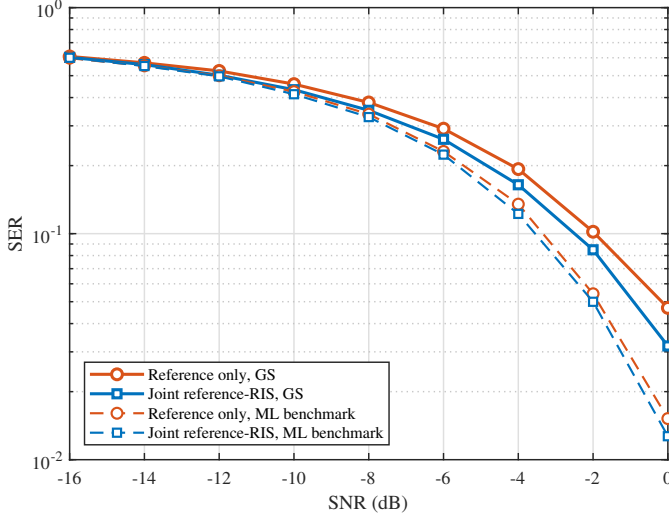
Fig. 16. SER of the proposed reference-assisted GS detector and the ML benchmark under equal-overhead reference-only and joint reference-RIS measurement diversity.
