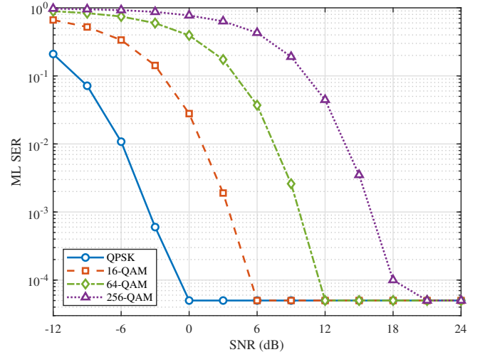
Fig. 10. ML SER for QPSK, 16-QAM, 64-QAM, and 256-QAM under perfect CSI. Zero-error points are displayed at the half-event level.
