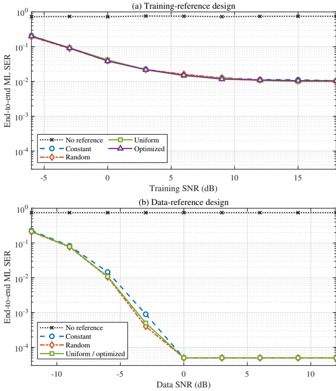
Fig. 12. End-to-end ML SER versus (a) training SNR for different training-reference designs at a data SNR of -6 dB and (b) data SNR for different data-reference designs at a training SNR of 12 dB. Zero-error points are displayed at the half-event level.
