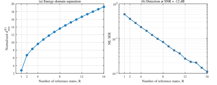
Fig. 14. Effect of the number of phase-shifted reference states on (a) the normalized energy-domain minimum distance and (b) ML detection.
