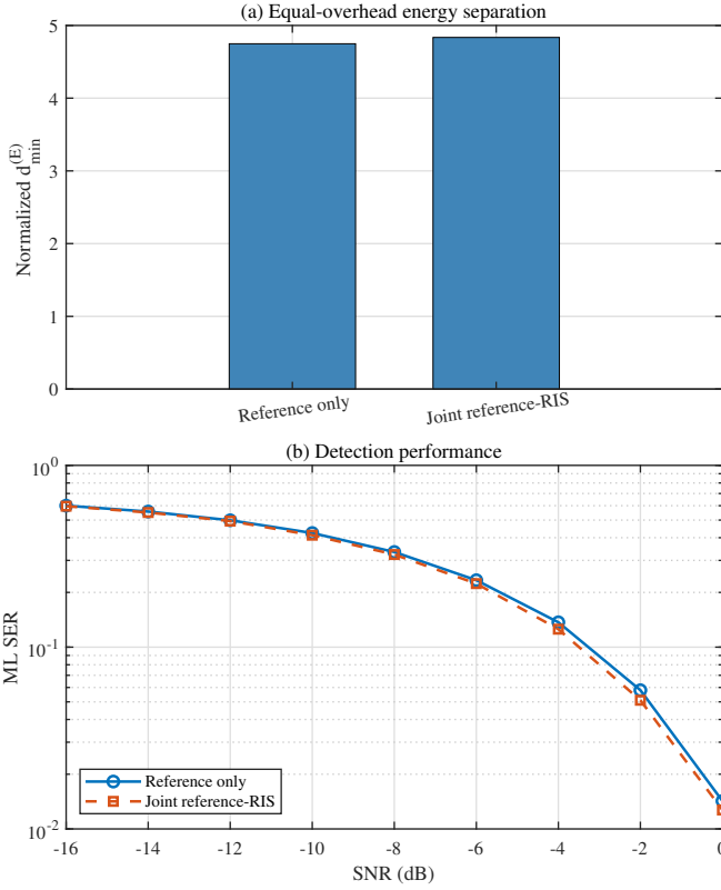
Fig. 16: Equal-overhead comparison of reference-only and joint reference-RIS measurement diversity: (a) normalized minimum distance and (b) ML SER.
