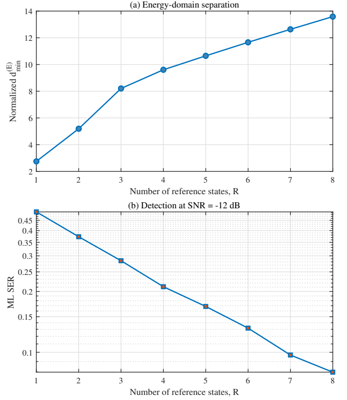
Fig. 14: Effect of the number of phase-shifted reference states on (a) the normalized energy-domain minimum distance and (b) ML detection.
