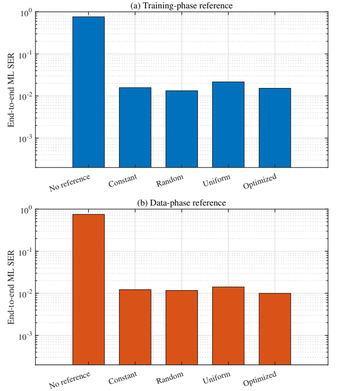
Fig. 12: End-to-end ML SER for different (a) training-phase and (b) data-phase reference designs.
