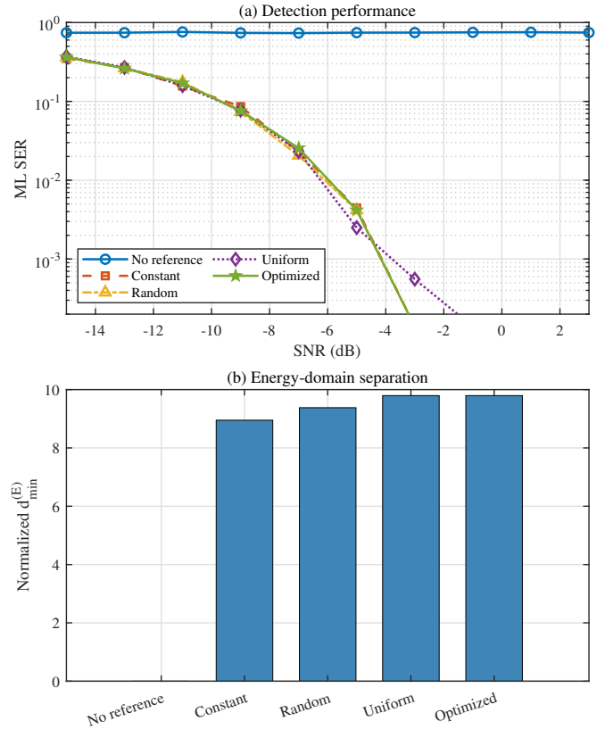
Fig. 7: Effect of the data-phase reference: (a) ML SER and (b) normalized energy-domain minimum distance.
