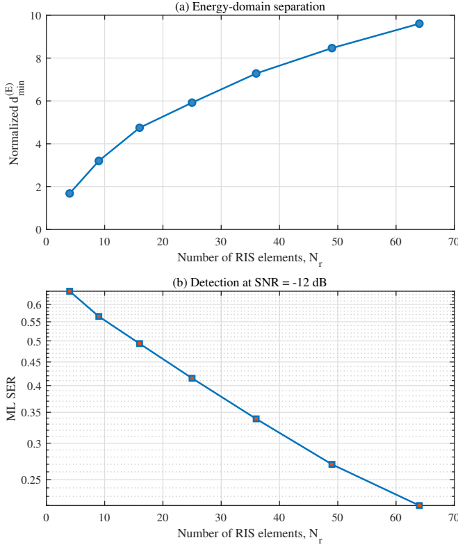
Fig. 13: Effect of the number of RIS element-level observations on (a) the normalized energy-domain minimum distance and (b) ML detection.
