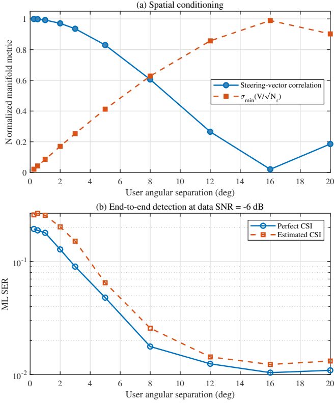
Fig. 15: Effect of user angular separation on (a) array-manifold conditioning and (b) end-to-end ML detection.
