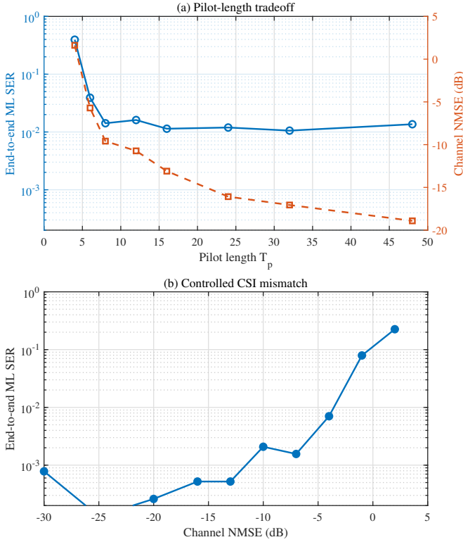
Fig. 11: Effect of channel-estimation accuracy on end-to-end ML detection: (a) pilot-length tradeoff and (b) controlled CSI mismatch.
