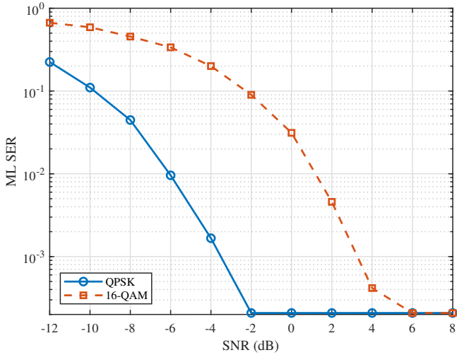
Fig. 9: ML SER for QPSK and 16-QAM under perfect CSI.
