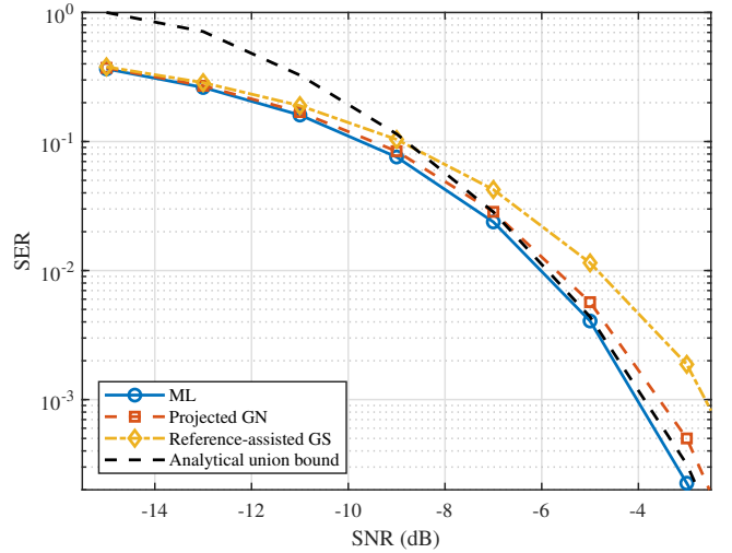
Fig. 7. SER of different symbol detectors under perfect CSI, averaged over 10^5 trials per SNR, and the analytical distance-spectrum union bound.
