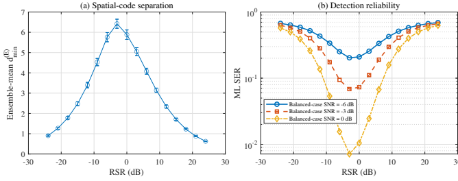
Fig. 11. Effect of the reference-to-signal energy ratio under a fixed total incident-energy budget: (a) ensemble-mean minimum energy distance over balanced spatial phase maps and (b) perfect-CSI ML SER at three balanced-case SNRs. Error bars show one standard deviation across phase maps.
