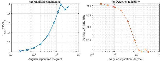
Fig. 10. Effect of user angular separation on (a) array-manifold conditioning and (b) perfect-CSI ML detection at -6 dB.
