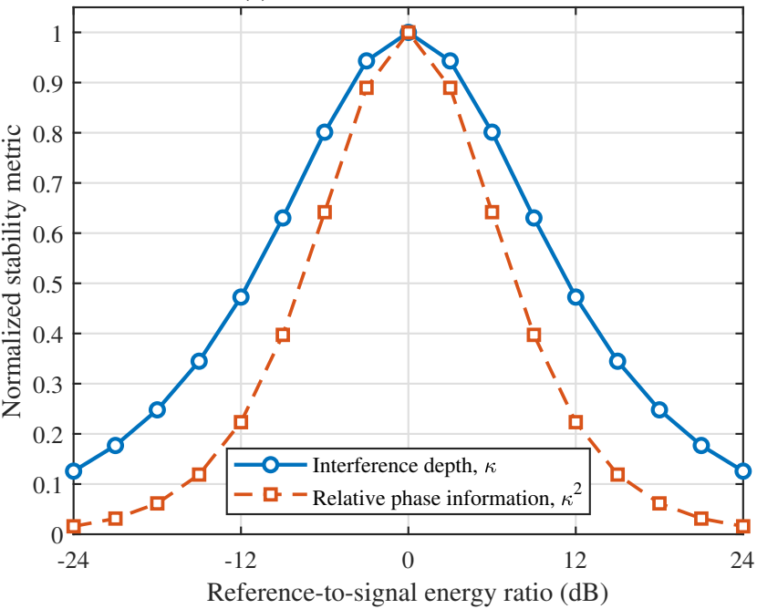
(a) Phase-sensitive interference
